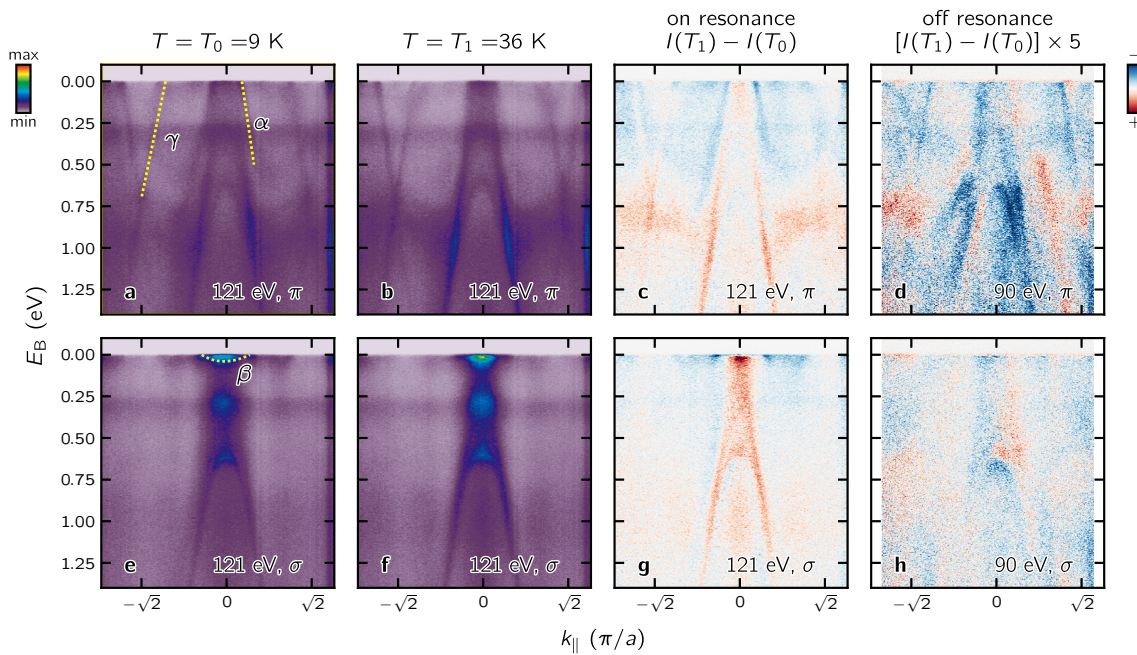
Fig. 2. (Color online) Zone corner band structure from Si-terminated Fermi surface. (a, b), (e, f) Band structure along the Z- Y_1 directions recorded with linear horizontal ( \pi ) and vertical ( \sigma ) light polarization for temperatures as indicated. (c, d), (g, h) Intensity difference I(36\text{ K}) - I(9\text{ K}) for the two polarizations at the resonance and off-resonance. The color scale is organized so that white indicates no difference, red indicates intensity gain and blue intensity loss upon heating. The color scale of the off resonance difference spectra (d, h) has been enhanced by 500% in order to make features visible at all. On the resonance, loss and gain traces the band structure whereas the off-resonance differences are generally a factor of 5 weaker and appear rather random.
