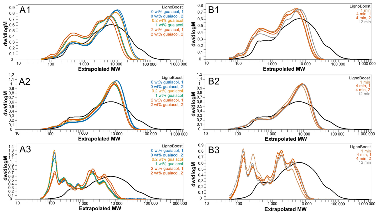
Figure 4: Molecular weight distributions of the char (1), PS (2) and ASO (3) fractions at 4 min residence time and varying mass fractions of guaiacol in the feed (A), and with 2 wt% guaiacol in the feed at different residence times (B). The unit is Da.
