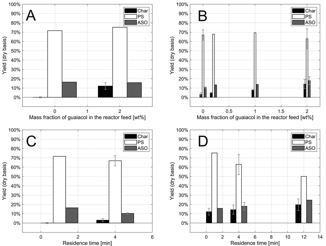
Figure 3: Yields of product fractions run at average reactor temperatures and pressures of 288–301 °C and 214–251 bar at varying mass fractions of guaiacol in the feed at 1 min (A) and 4 min (B) residence times, respectively, and at varying residence times with 0 wt% (C) and 2 wt% (D) guaiacol in the feed, respectively.
