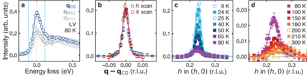
Figure 4.4: Elastic scans through the charge order. a RIXS spectra collected at the charge order wave vector q_{CO} and at two background positions q_{BG1} = (0.346, 0) and q_{BG2} = (0.129, 0) . Light blue vertical dashed lines indicate the energy window for the elastic intensity integration. b Elastic scans along h and k directions. c, d Elastic h scans recorded at different temperatures with linear background subtracted. The filled and open markers represent data collected at ADDRESS and I21, respectively. Solid lines are Gaussian fits. Figure adapted from Ref. [98].
