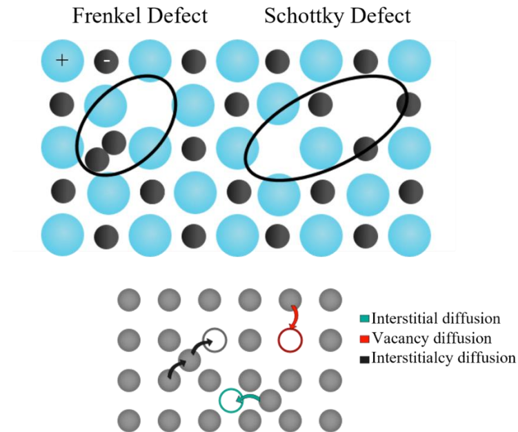
Figure 3.3: Illustration of Frenkel and Schottky defects for stoichiometric oxides and diffusion mechanisms of the ions in the crystal lattice.
