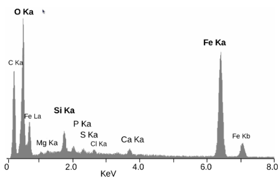
Figure 7.4: EDX spectrum.
