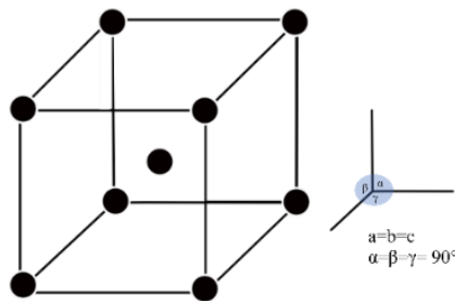
Figure 4.1: Body-centered cubic (BBC) crystal structure.
