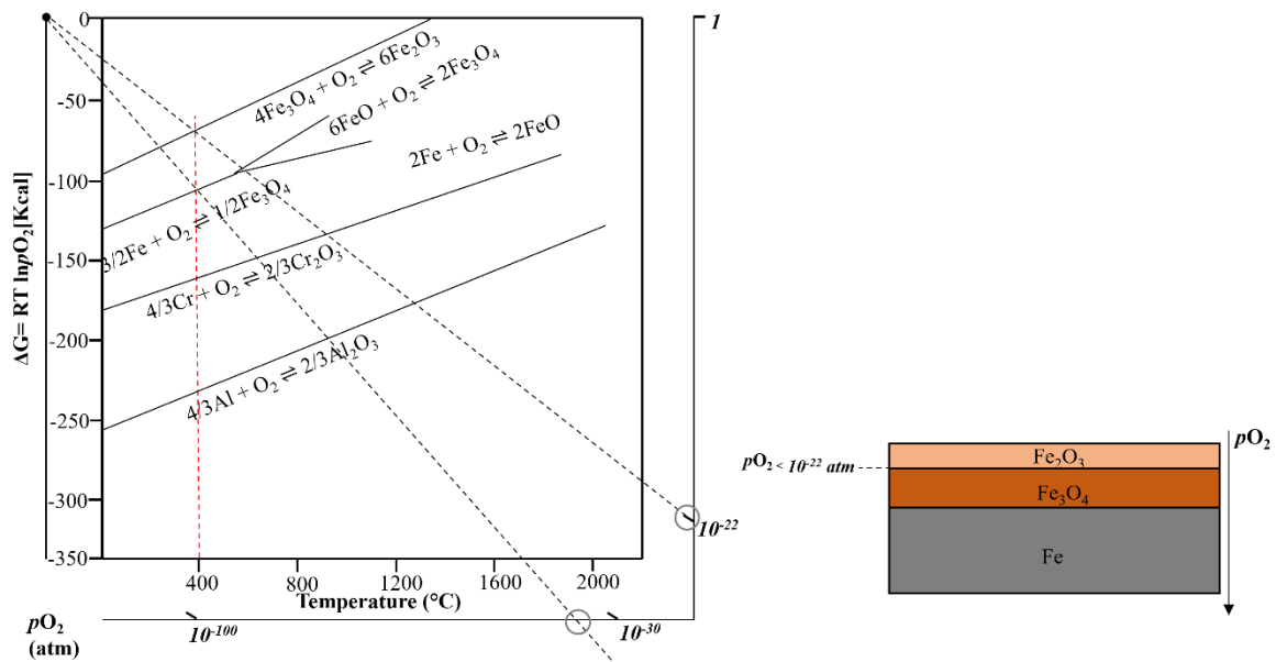
Figure 3.1: Left panel: Ellingham-Richardson diagram, adapted from [76]. Right panel: the multilayer oxide scale formed in pure Fe at 400°C. The position of the oxide scale is determined by the pO_2 .
