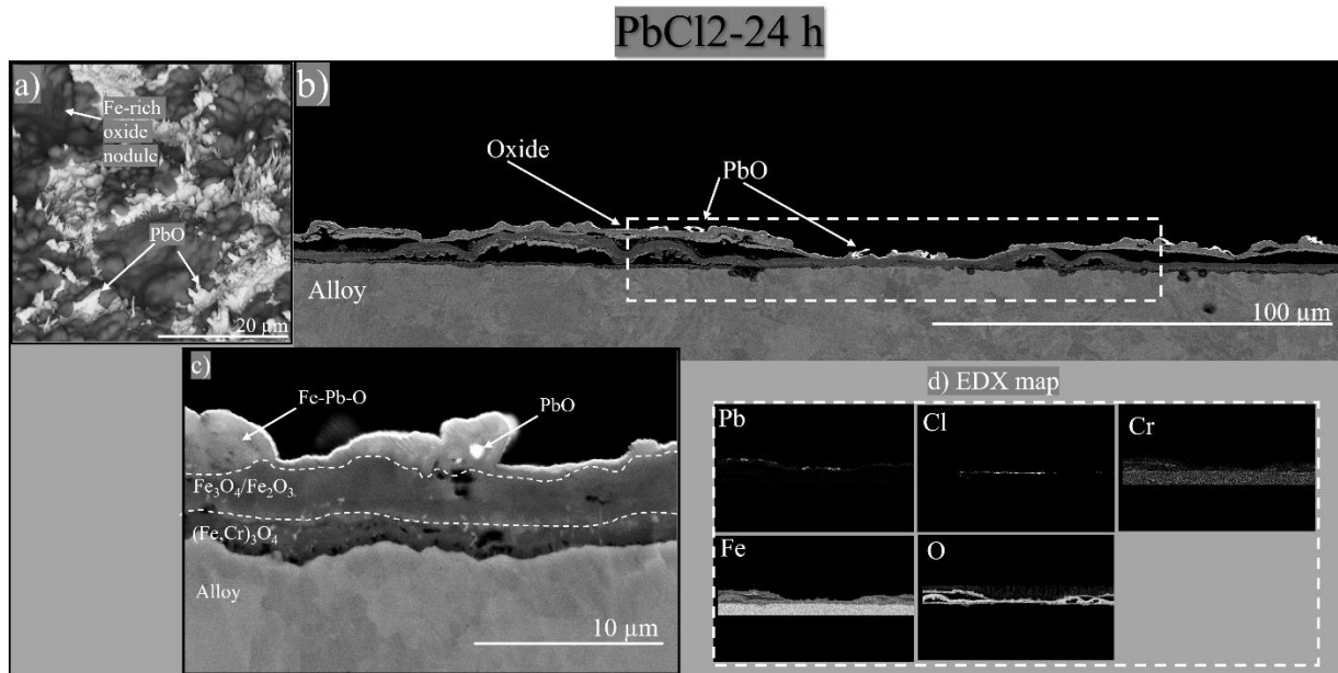
Figure 8.12: SEM BSE image of T22 exposed at 400°C in \text{PbCl}_2(\text{s}) + 5\%\text{O}_2 + 20\%\text{H}_2\text{O} + \text{N}_2 bal. for 24 hours. (a) Plan view image; (b) Cross-section; (c) Section with Fe-Pb-O formation; (d) EDX map of highlighted area in (b).
