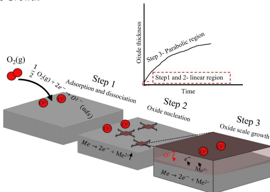
Figure 3.2: Oxide growth mechanism.
