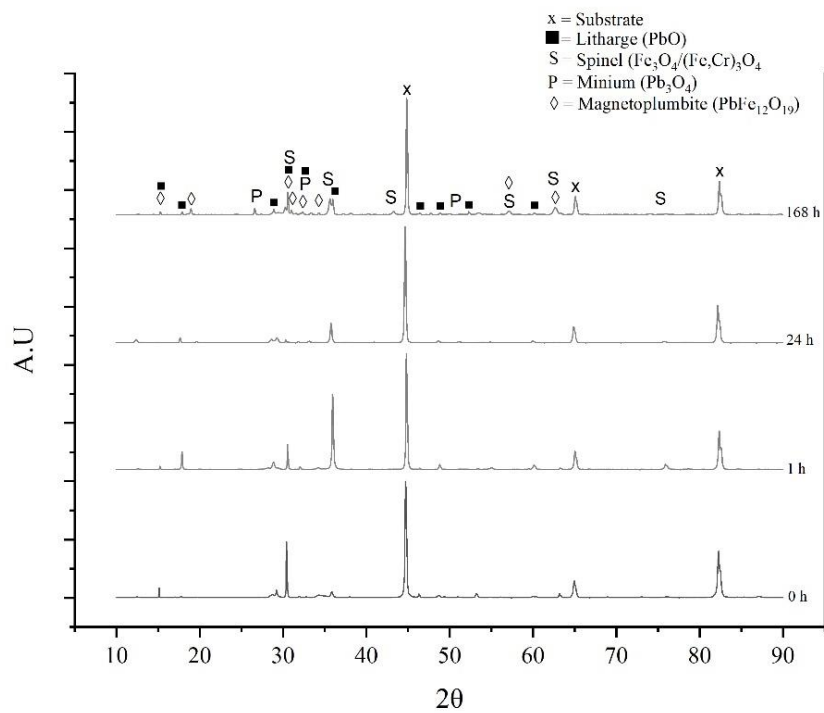
Figure 8.15: XRD spectra for samples exposed to PbO.
