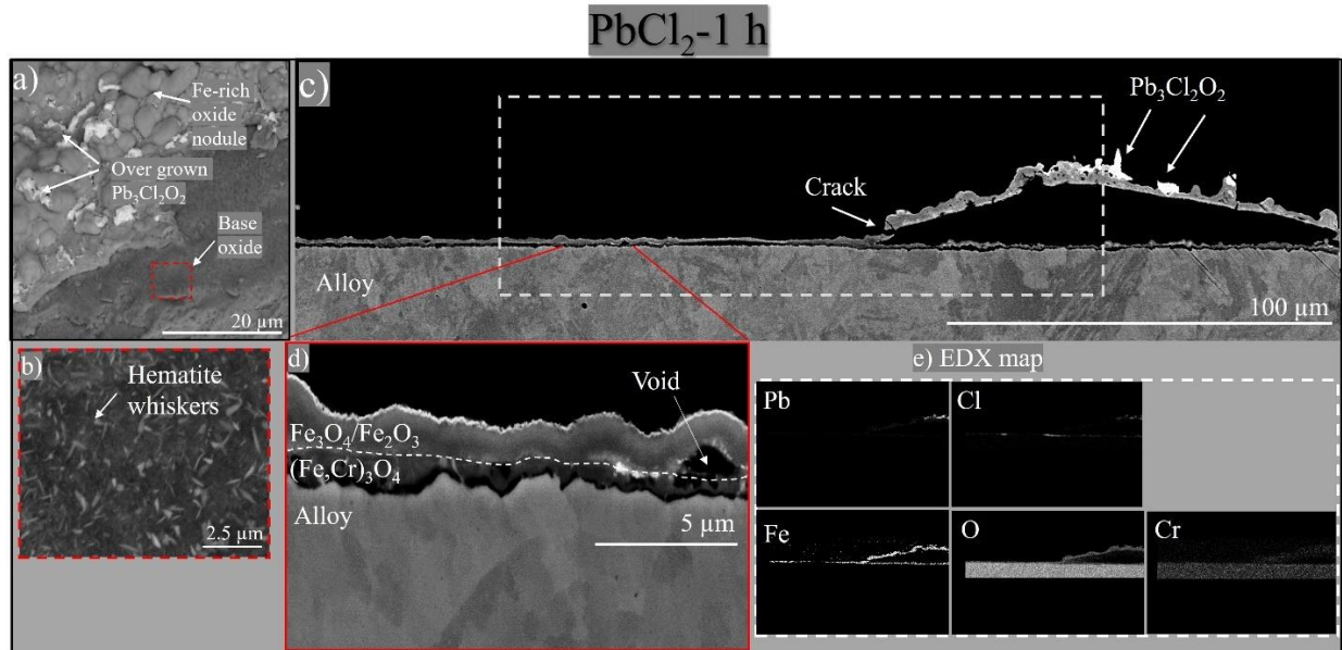
Figure 8.10: SEM BSE image of T22 exposed at 400°C in PbCl 2 (s) + 5%O 2 + 20% H 2 O + N 2 bal. for 1 hour. (a) Plan view image; (b) Highlighted area in (a); (c) Cross-section; (d) Higher magnification of selected area; (e) EDX map of highlighted area in (c).
