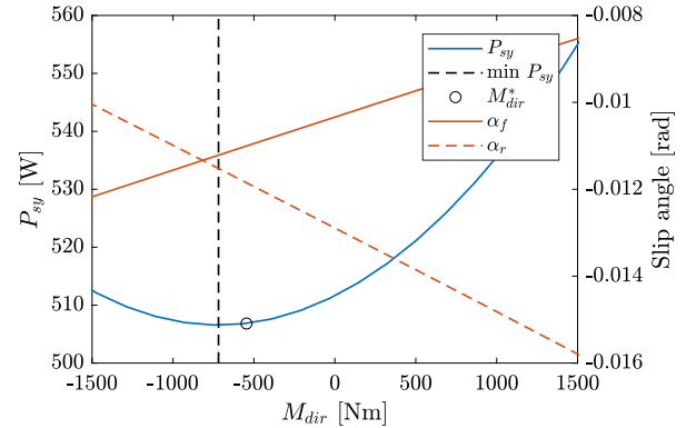
Fig. 4: Lateral tire slip loss and tire slip angles for the oversteered case K_{us} = -0.0009 .
