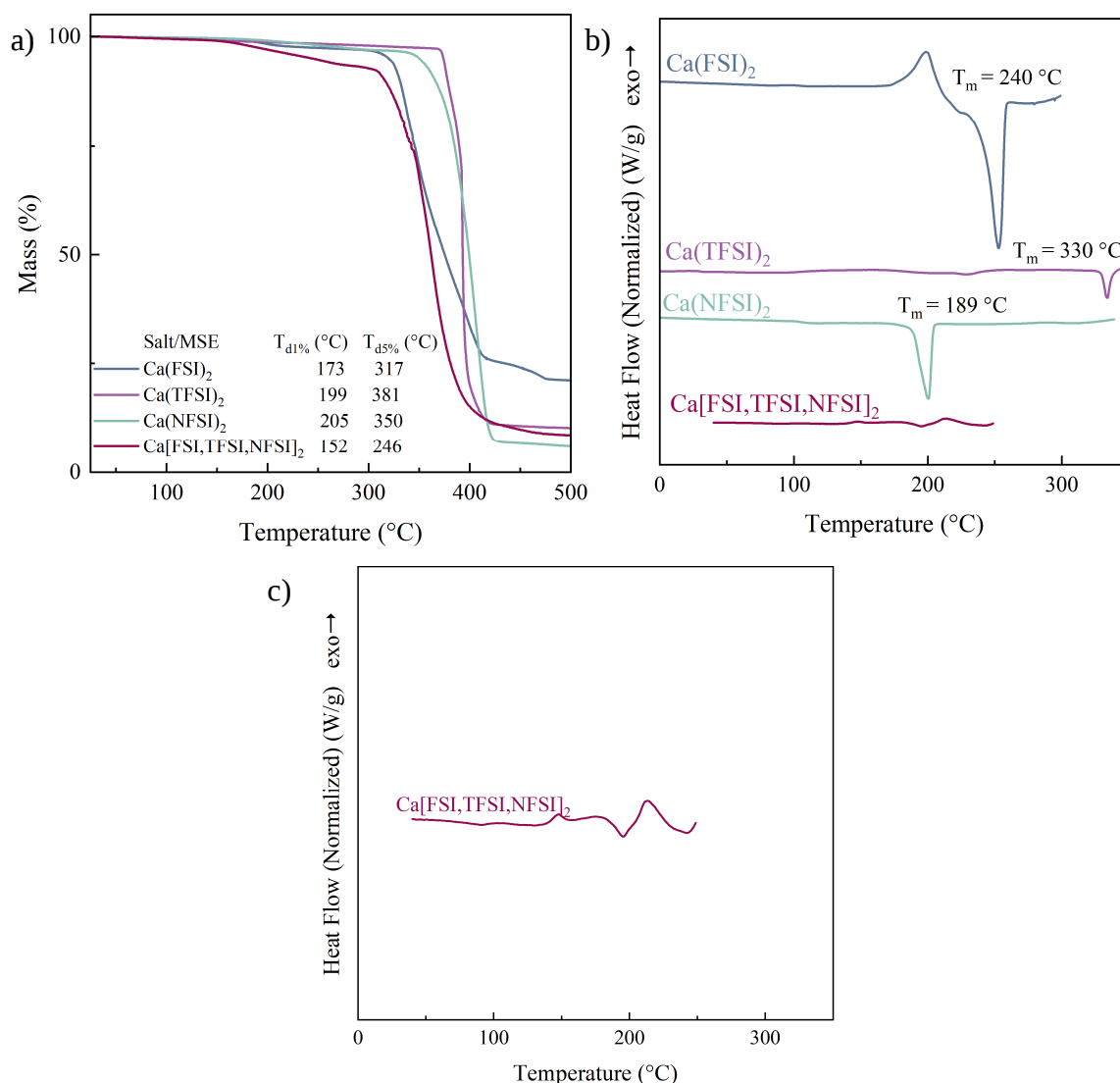
Figure 5.1. Graphs of single Ca-salt and the MSE \text{Ca}[\text{FSI}, \text{TFSI}, \text{NFSI}]_2 where a) show TGA traces of the decomposition behaviour, b) show DSC traces of the melting behaviour and c) close-up of \text{Ca}[\text{FSI}, \text{TFSI}, \text{NFSI}]_2 .
