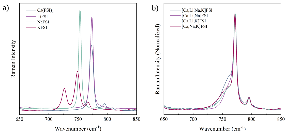
Figure 5.6. Raman spectra of a) single salts and b) MSEs in the spectral range between 650-850 \text{cm}^{-1} .
