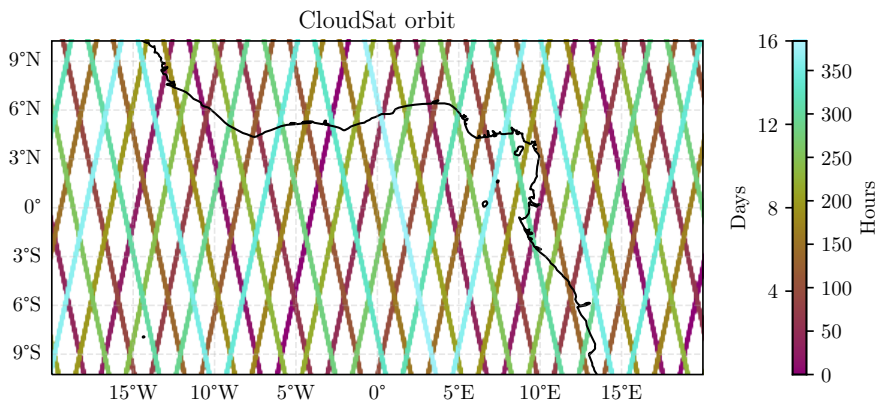
Figure 2.4: One full CloudSat repeat cycle for a region centred at 0° latitude and longitude. The cross-track field of view is not to scale, therefore even a larger part of the region is unobserved by CloudSat. The colours indicate the elapsed time since a hypothetical start time of observation.
