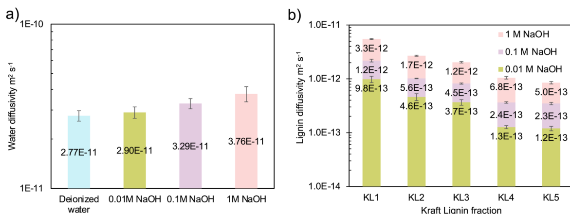
Figure 13 a) Diffusivity of tritium-labeled water through the 50 kDa MWCO membrane at various levels of alkalinity. b) Variation in diffusivity of fractionated lignin under different alkaline conditions.
