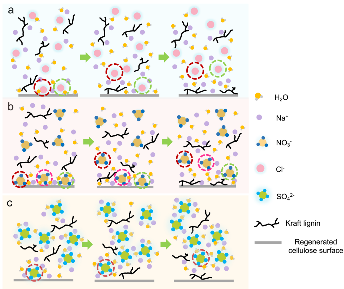
Figure 16 Illustration depicting lignin adsorption in the presence of different salts: a) \text{NaCl} , b) \text{NaNO}_3 , and c) \text{Na}_2\text{SO}_4 . The sequence from left to right demonstrates the arrangement of ions in the system. Notably, chaotropic (weakly hydrated) nitrate ions (b) tend to selectively organize themselves on the cellulose surface, while kosmotropic (highly hydrated) sulfate ions (c) are primarily distributed within the bulk water. The presence of nitrate ions on the surface prompts a more ordered configuration of water molecules near the membrane. Upon adsorption of lignin molecules onto the cellulose surface, the ions initially positioned on the surface are released into the surrounding solution. This ion release leads to an increase in the system's entropy.
