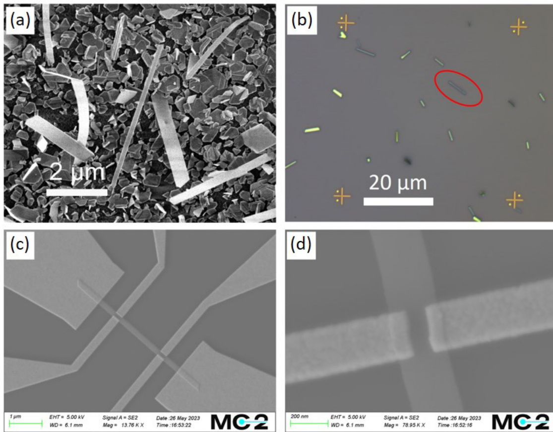
Figure 5. (a) Secondary electron SEM image of grown freestanding \text{Bi}_2\text{Se}_3 nanoribbons on a glass substrate. (b) Optical image of transferred nanoribbons to \text{Si}/\text{SiO}_2 substrate. The red circle highlights the nanoribbon (15 nm thick) selected for further fabrication. (c) SEM image of \text{Bi}_2\text{Se}_3 nanoribbon-based (from (b)) device with patterned electrodes for the Hall-effect measurement; (d) Hall bars overlapping the \text{Bi}_2\text{Se}_3 nanoribbon; this configuration requires a correction factor g when calculating the n_{3\text{D-Hall}} concentration.
