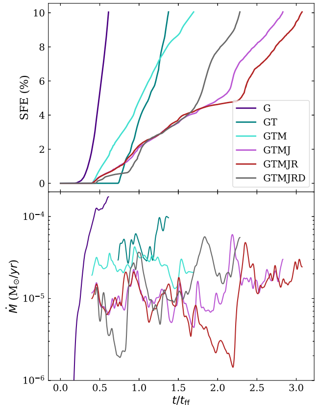
Figure 13. Figure 2 with runs GTMJ and GTMJRD, which includes decaying turbulence instead of continuous turbulence driving.
