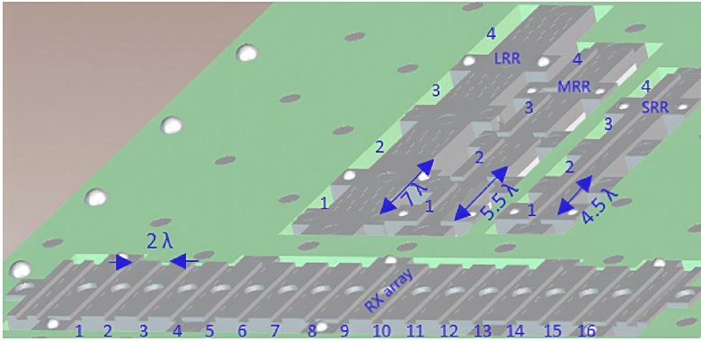
Figure 2.7: Simultaneous multi-mode automotive imaging radar system using waveguide slot arrays. [56].
