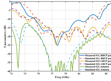
Figure 18: Measured and simulated results of the proposed planar array.
