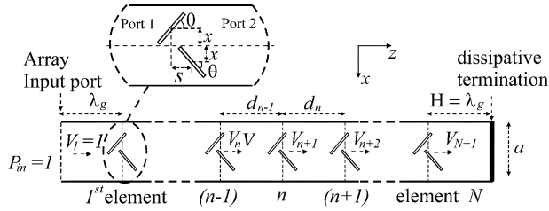
Figure 2.10: Proposed travelling wave CP linear array based on inclined waveguide slots [59].
