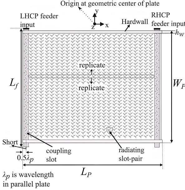
Figure 2.11: Proposed dual circularly polarized travelling-wave antenna using parallel plate slot pairs [60].
