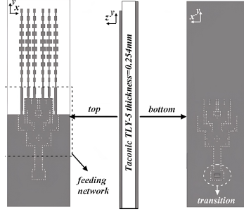
Figure 2.2: Configuration of the proposed antenna [43].
