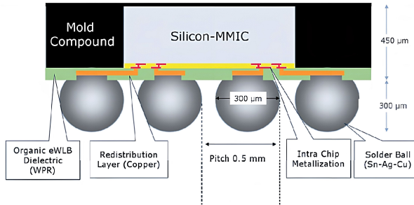
Figure 3.1: Cross section of an eWLB package [69].
