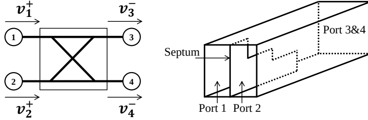
Figure 2.12: Illustration of a four-port septum polarizer.
