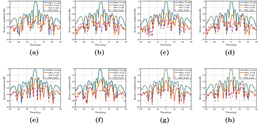
Figure 20: Simulated and measured realized gain patterns of the planar array: (a) RHCP in x - z at 76.5 GHz; (b) RHCP in x - z at 78.5 GHz; (c) RHCP in y - z at 76.5 GHz; (d) RHCP in y - z at 78.5 GHz; (e) LHCP in x - z at 76.5 GHz; (f) LHCP in x - z at 78.5 GHz; (g) LHCP in y - z at 76.5 GHz; (h) LHCP in y - z at 78.5 GHz.
