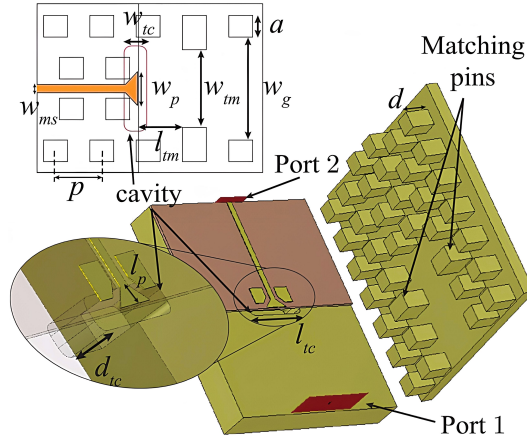
Figure 3.11: Configuration of the proposed microstrip-to-waveguide in-line transition [33].
