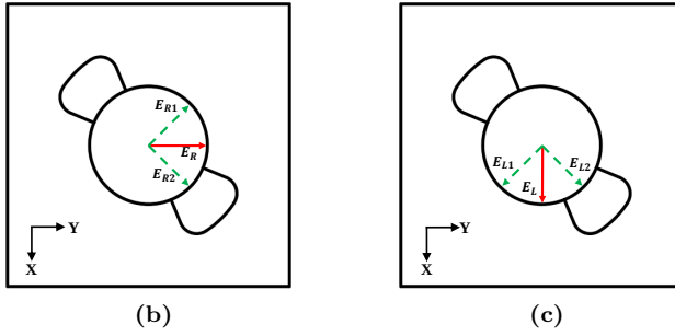
Figure 2.15: Illustration of double grooved circular waveguide polarizer.
