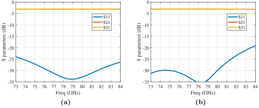
Figure 10: Simulated S parameters of the (a) E-plane T-junction and (b) H-plane T-junction power dividers.
