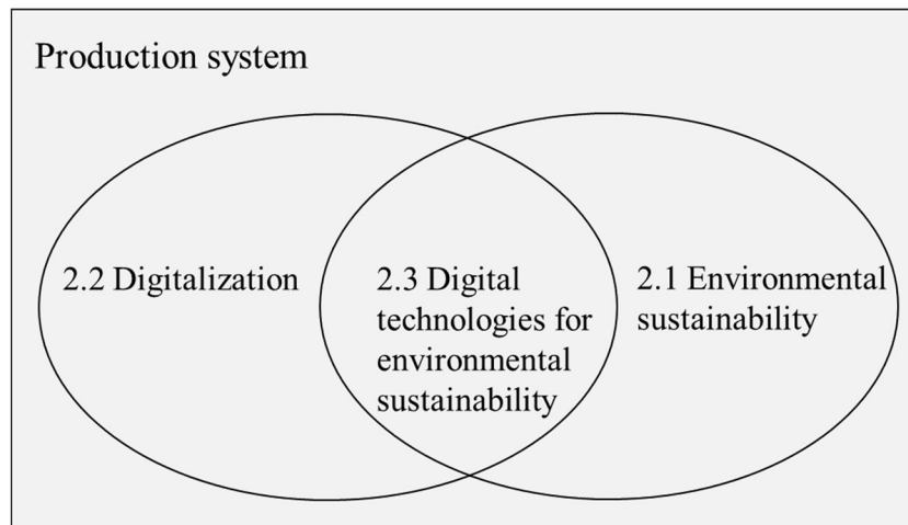
Figure 2. Research framework.
