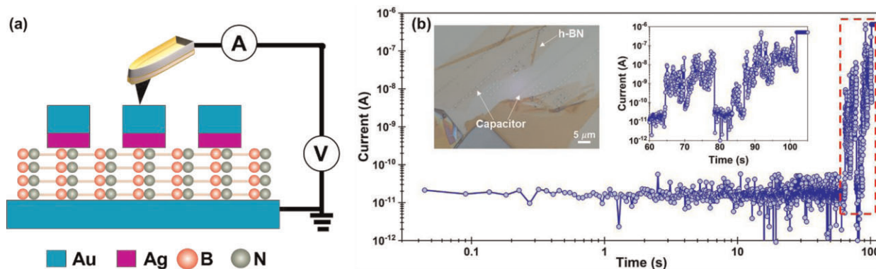
Fig. 1. (a) Schematic diagram showing a cross-sectional view of a Au/h-BN/Ag capacitor and the electrical connections for the CAFM measurements. (b) TDDB characteristics measured on a 500 nm \times 500 nm capacitor showing the evolution of leakage current with time. The applied electrical field is 7.5 MV/cm. The inset image shows an optical micrograph of the fabricated capacitor.
