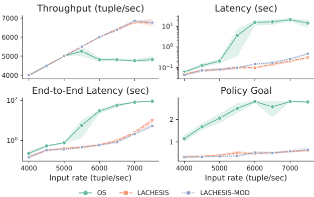
Figure 7: Results with the LR query on STORM.
