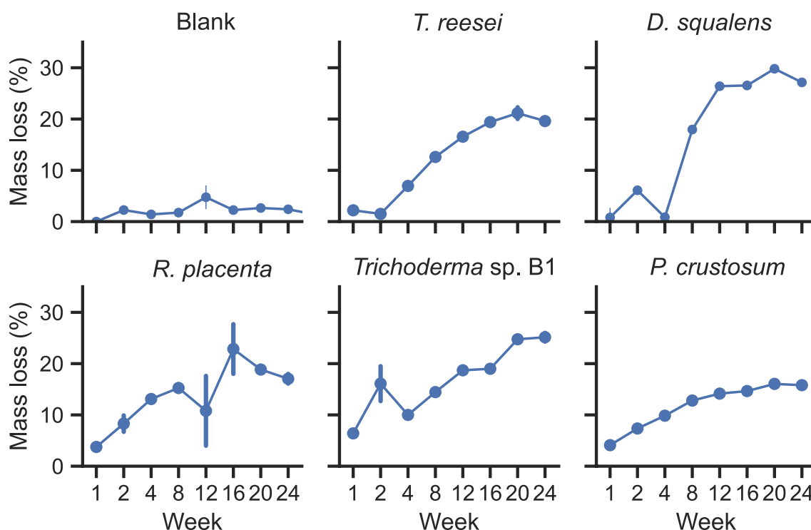
Figure 3.8. Growth of filamentous fungi during six months (24 weeks) using spruce bark as the sole carbon source. Measurements were based on overall mass loss. No fungus was added to the blank (control) sample. The plates were incubated at 20°C. Values correspond to the mean of duplicate biological experiments. Adapted from Paper II.
