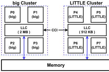
Fig. 8. Hardware platform.
