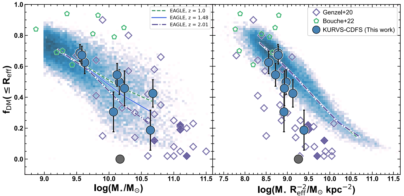
Figure 8. Dark matter fraction within the disc effective radius for high-redshift star-forming galaxies as a function of stellar mass (left) and stellar mass surface density (right). The 2D density histogram shows measurements for simulated EAGLE galaxies at z = 1.0, 1.48 , and 2.01 . The coloured lines show the running median at each redshift in EAGLE. The open green pentagons show the Bouché et al. (2022) sample of z \sim 0.9 star-forming galaxies. The open purple diamonds indicate the Genzel et al. (2020) sample at 0.67 \lesssim z \lesssim 2.45 , with filled symbols highlighting the sources that are in the same redshift range as our sample. Large filled circles represent rotationally supported galaxies in KURVS-CDFS, with the grey data point indicating a source whose kinematics are not well described by GALPAK 3D . Simulated EAGLE galaxies show a trend of decreasing dark matter fraction with increasing stellar mass, albeit with large scatter. Observed galaxies follow the same trend. There is a much tighter anticorrelation between the dark matter fraction and the stellar mass surface density in EAGLE. Observations follow a similar trend up to \log(\Sigma_*/M_\odot/\text{kpc}^{-2}) \sim 9.2 . At higher stellar mass surface densities, however, EAGLE overpredicts the dark matter fraction of observed galaxies by a factor of \sim 3 .
