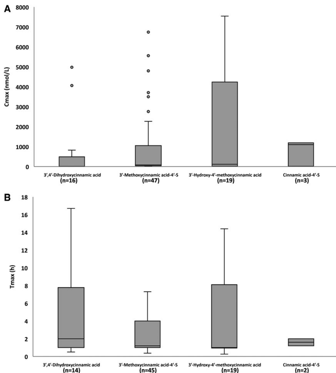
FIG. 3. Box plot for C_{\max} (nM) (A) and T_{\max} (h) (B) for 4 out of 10 main C_6-C_3 cinnamic acids quantified in blood sample after the intake of HCAs and/or other (poly)phenols (see Supplementary Table S3 for the complete list of the main 18 plasma HCA metabolites). The main plasma circulating compounds were selected based on a normalized C_{\max} value \geq 0.4 nM, calculated using at least three biological replicates deriving from at least two articles. n indicates the number of biological replicates collected for the same HCA metabolite and for the same pharmacokinetic parameter. Metabolites are named according to Kay et al. (2020). S, sulfate.
