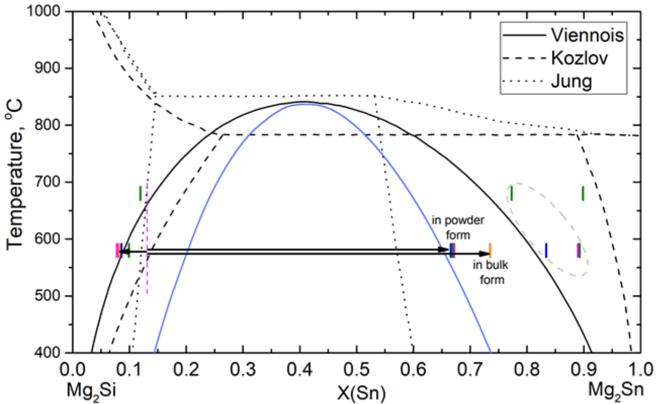
Figure 18. Available phase diagrams [11-14] of \text{Mg}_2\text{Si} - \text{Mg}_2\text{Sn} and formed phases in the samples of the current work, which were treated inside the miscibility gap:
