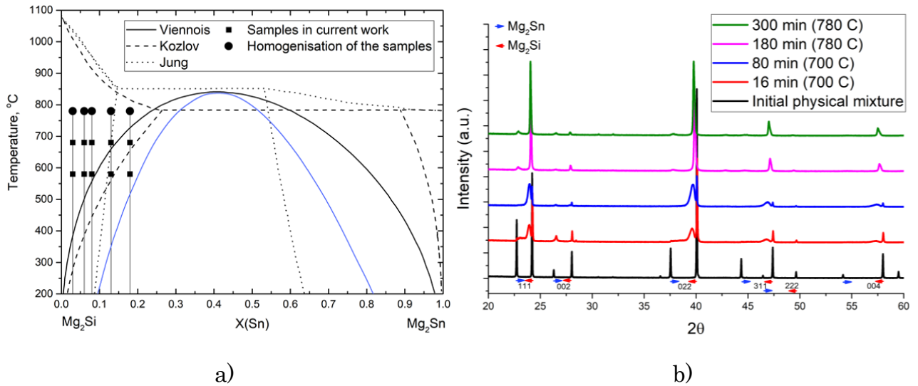
Figure 14. Existing quasi-binary phase diagrams of \text{Mg}_2\text{Si} - \text{Mg}_2\text{Sn} [11-14] highlighting experiments done in Paper II (blue solid curve shows an approx. shape of the spinodal region according to Viennois et al. [14]) (a) and ex-situ XRD analysis of the \text{Mg}_2\text{Si}_{0.87}\text{Sn}_{0.13} solid solution formation (b).
