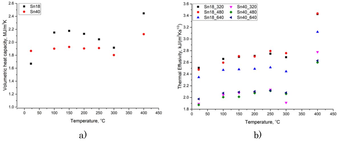
Figure 25. Heat capacity per unit volume (a) and thermal effusivity (b) obtained by Hot Disk methods.
