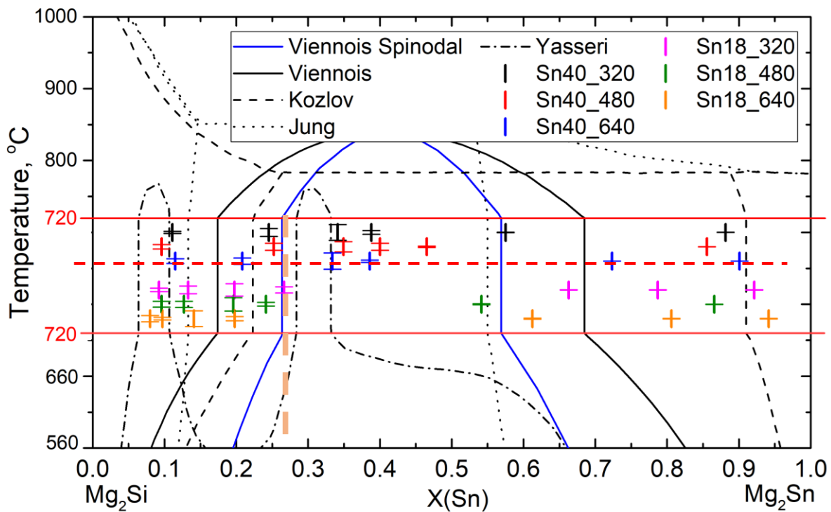
Figure 21. \text{Mg}_2(\text{Si}_{1-x}\text{Sn}_x)_{0.975}\text{Bi}_{0.025} phases in the \text{Mg}_2(\text{Si}_{0.82}\text{Sn}_{0.18})_{0.975}\text{Bi}_{0.025} and \text{Mg}_{2.2}(\text{Si}_{0.6}\text{Sn}_{0.4})_{0.975}\text{Bi}_{0.025} samples after homogenization at 720 °C in SPS.
