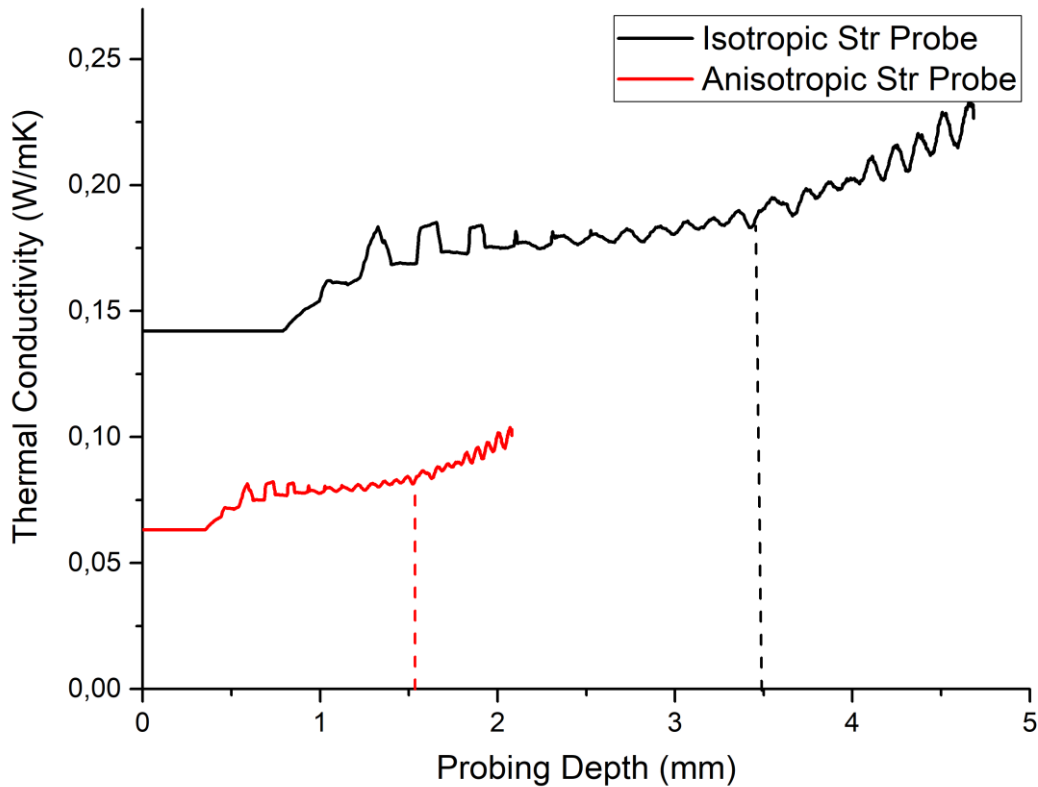
Figure 32. Thermal conductivity versus probing depth, acquired using the original method with (\rho c_p)_{\text{false}} and the new approach on a printing paper stack.
