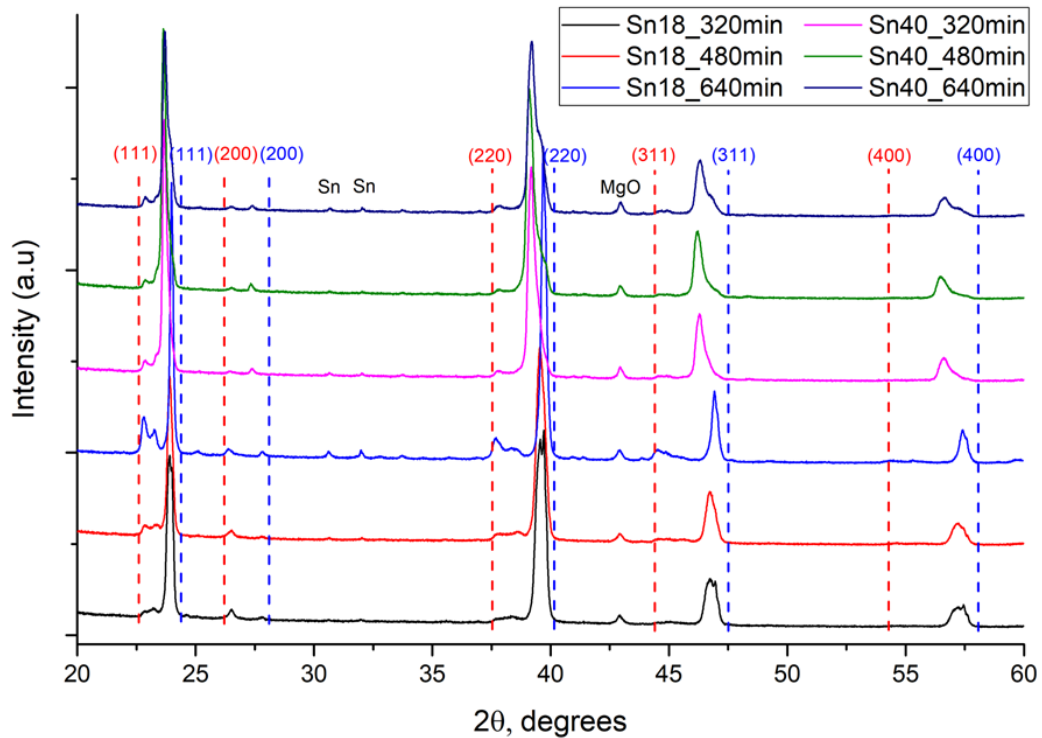
Figure 20. XRD patterns of \text{Mg}_2(\text{Si}_{0.82}\text{Sn}_{0.18})_{0.975}\text{Bi}_{0.025} and \text{Mg}_2(\text{Si}_{0.6}\text{Sn}_{0.4})_{0.975}\text{Bi}_{0.025} after SPS sintering at 720^\circ\text{C} during different dwelling time.
