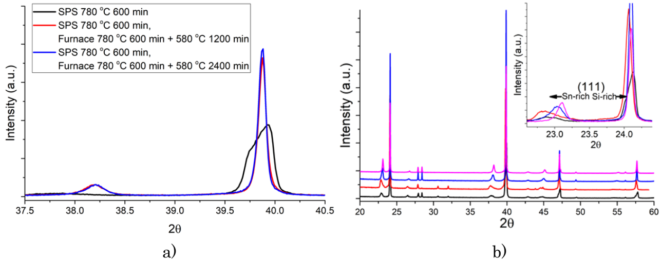
Figure 23. XRD patterns for \text{Mg}_2\text{Si}_{0.87}\text{Sn}_{0.13} : a) phase separation during treatment at 580 °C (reflection 220); (b) experiencing different cooling rates: quick cooling (black), slow linear cooling to 400 °C (red), slow exponential to RT (blue) and slow exponential from 580 °C to RT (magenta).
