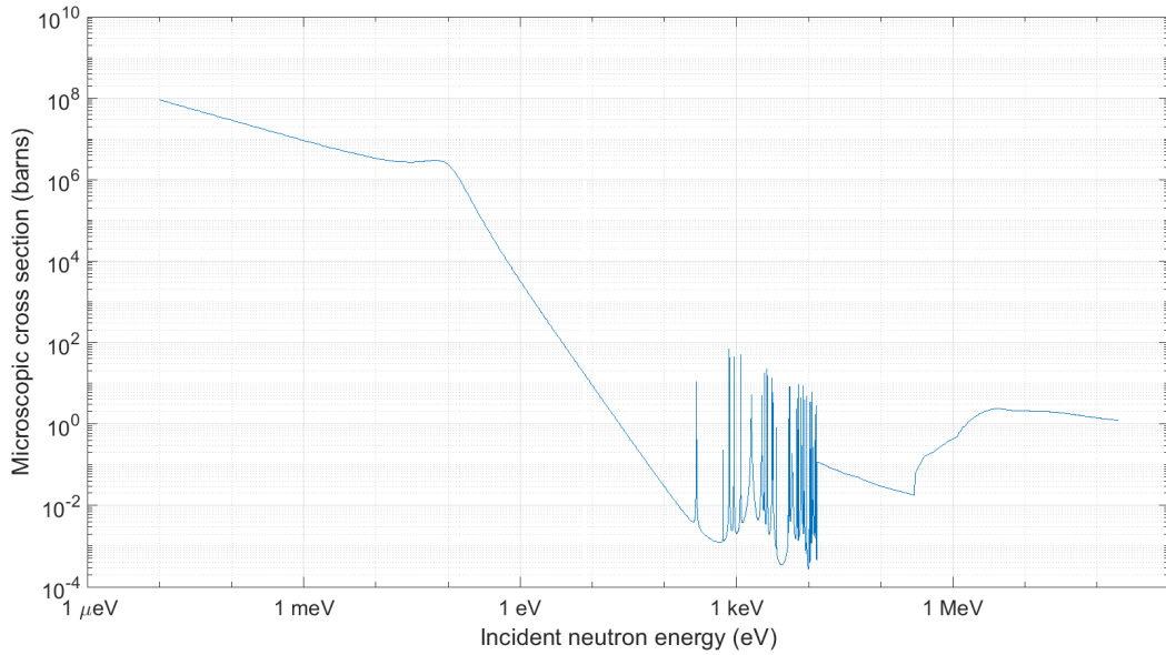
Figure 1.3: Xenon absorption cross section as a function of neutron energy
