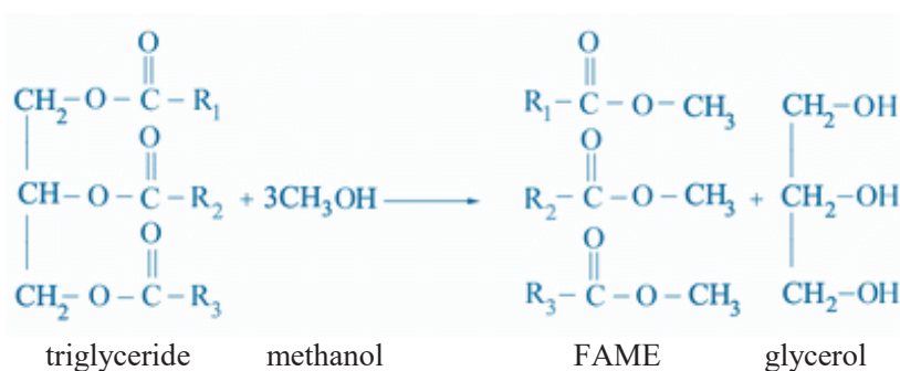
Figure 2. Transesterification reaction to achieve biodiesel production through a chemical or enzymatic reaction of triglyceride present in plant oils and methanol to form FAMES and glycerol as a by-product.
