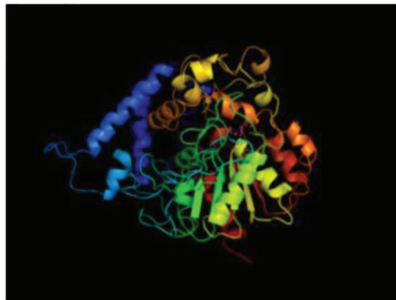
Figure 20. Prediction of tertiary structure of the Eeb1p wild-type and selected variant (E-v4). Sequences are presented in rainbow spectrum from protein head by N-terminus (dark blue) to protein tail by C-terminus (dark red). The active site is marked with gray spots of the residues of the catalytic triad (S251, D399 and H428). Reference: Kelley and Sternberg, 2009.
