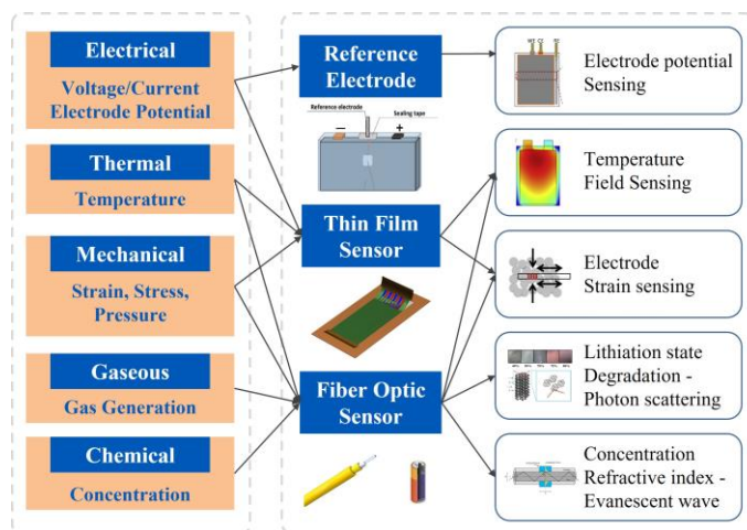
Fig. 8. Categories and representative sensors for battery monitoring
