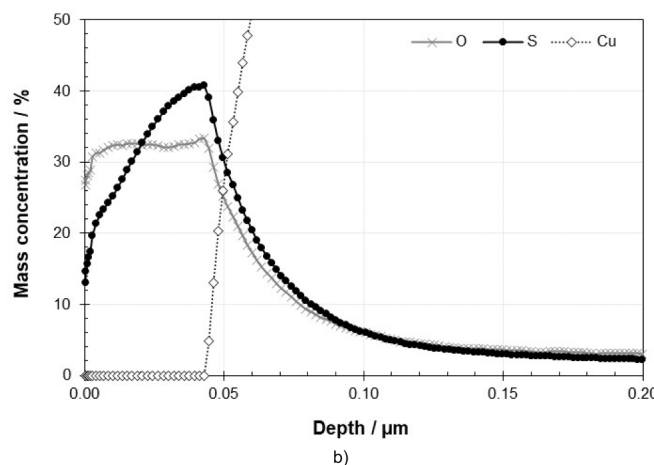
Fig. 10. Elemental depth profiles of oxygen, sulphur and copper for pre-oxidized specimen exposed to simulated groundwater with 32 mg/L sulphide addition. a) Profile down to the depth of 1.0 μm. b) Zoomed profile down to the depth of 0.2 μm.
