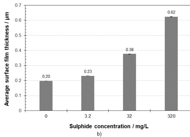
Fig. 5. a) Weight loss of the specimens during the test and by the corrosion product removal after the test. b) Average thickness of the corrosion product film deduced from weight loss of the specimens by corrosion product removal.
