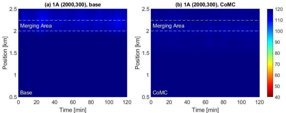
Fig. 6. Speed contour.
