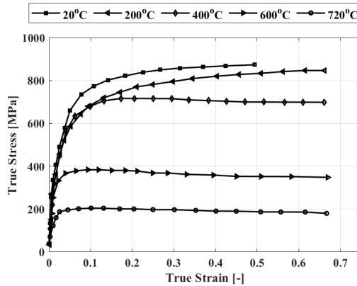
Figure 3.4: Stress-strain response of medium carbon steel [24] under quasi static loading at different temperatures.
