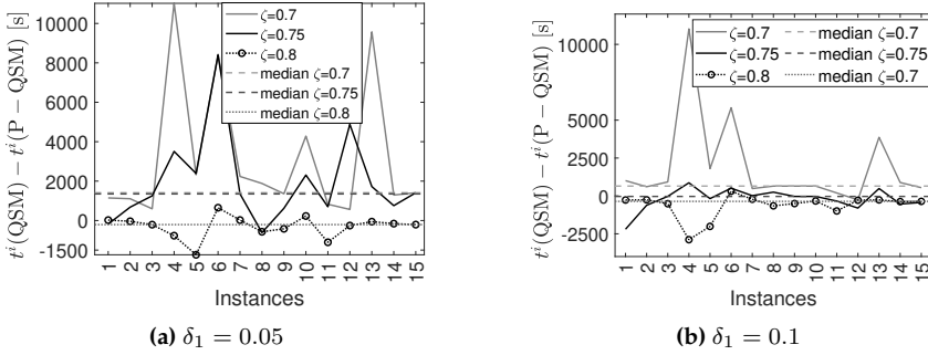
Figure 4.4: Difference of solution time for QSM and P-QSM [s] for threshold values \zeta \in \{0.70, 0.75, 0.80\} and varied the discretization \delta_1 \in \{0.05, 0.1\} used for the first objective function which is not integer-valued
