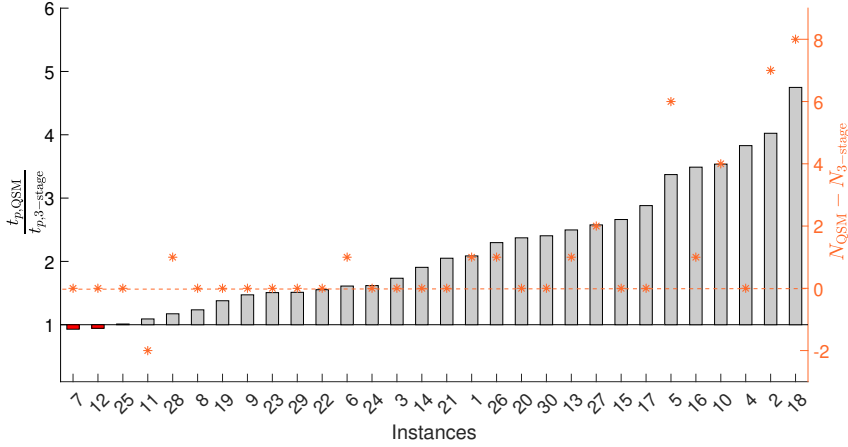
Figure 4.3: Left axis: Ratio of solutions times (grey bars; red bars for negative values). Right axis: Difference between the number of PRO-RE solutions identified by the QSM ( N_{QSM} ) and the 3-stage method ( N_{3-stage} ) (orange asterisk). All computed sets are minimal sets
