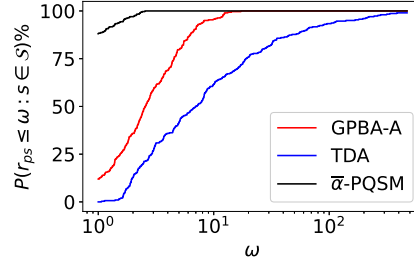
Figure 4.5: Performance profile for different algorithms using the ratio of solution time as the performance measure for multi-dimensional three-objective knapsack instances.
