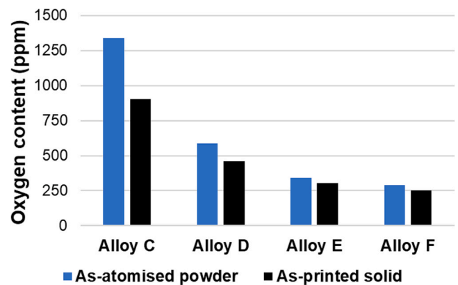
Fig. 13. Oxygen content in as-atomised powder and as-printed solid for all four variants. Testing done by combustion gas analysis.
