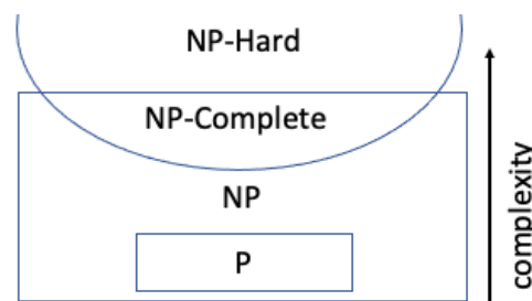
Figure 3.2: Diagram of intersection among classes P, NP, NP-complete and NP-hard problems. The least complex class of problems is P while the most complex one is NP-hard/complete.
