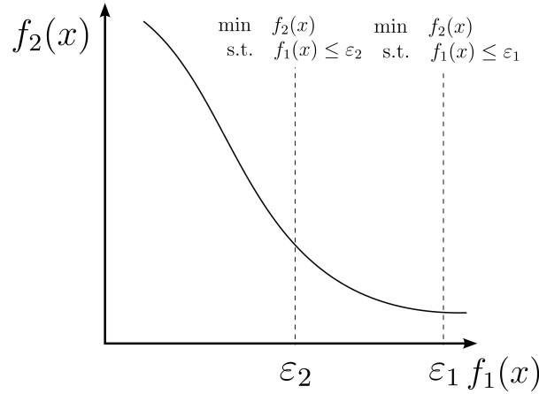
Figure 3.1: \varepsilon -constraint method for a (linear) bi-objective optimization problem. One objective is optimized while the other one is constrained by the values of \varepsilon . The distribution and number of \varepsilon values is a matter of choice. If we consider the range in between the smallest possible ( \varepsilon_{\min} ) and the largest possible ( \varepsilon_1 \geq \varepsilon_{\min} ) value of \varepsilon , then we update the \varepsilon_s := \varepsilon_{s-1} - \frac{1}{n}(\varepsilon_1 - \varepsilon_{\min}) , until \varepsilon_s \leq \varepsilon_k , where s is the index of the current \varepsilon , and n is the number of discrete epsilon values used.
