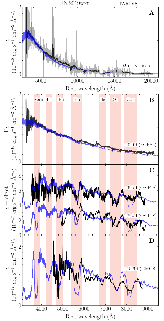
Fig. 8. Comparisons between our model spectra (blue) and observations (black). The observed spectra have been rebinned by a factor of 10 (using SPECTRES, Carnall 2017). Panel A: Comparison of the +0.9 d X-shooter spectrum with our best-fitting TARDIS model. Panel B: Comparison of the early FORS2 spectrum (+0.9 d), and our best-fitting TARDIS model. Panel C: Comparison of the two later OSIRIS spectra (+6.5 and +8.4 d) with their corresponding TARDIS models. The +6.5 d spectrum and model have been offset by 3 \times 10^{-17} \text{ erg s}^{-1} \text{ cm}^{-2} \text{ \AA}^{-1} , for clarity. Panel D: Comparison of the late-time GMOS spectrum (+15.6 d), and its corresponding TARDIS model. The vertical shaded bands in panels B, C and D correspond to regions of absorption in the observed spectra. The species dominating these same absorption features in our best-fitting TARDIS models have added to the top of each band in panel B.
