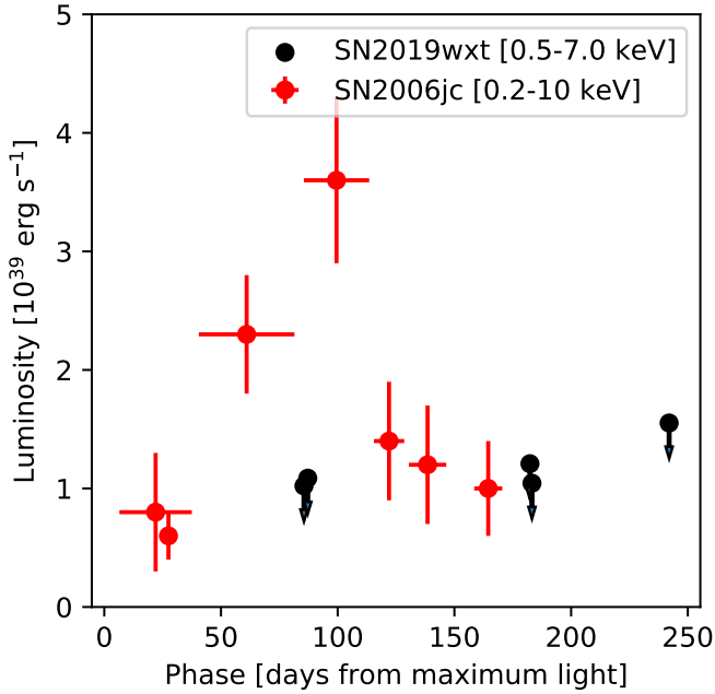
Fig. B.1. Chandra +ACIS upper limits to the x-ray luminosity of SN2019wxt, compared to the X-ray lightcurve of the Type Ibn SN2006jc. The Swift +XRT limit < 6.6 \times 10^{41} erg s ^{-1} at 0 d is more than two orders of magnitude shallower than the data plotted here, and hence not plotted.
