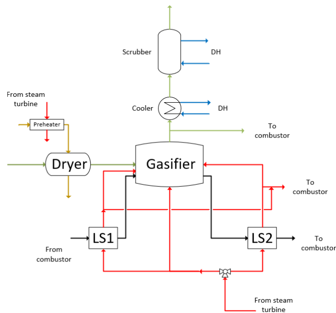
Figure B1: Schematic diagram of the retrofit assessed within the project. The same layout applies to the CFB and BFB reference plants. LS: loop seal. Source: [52]
