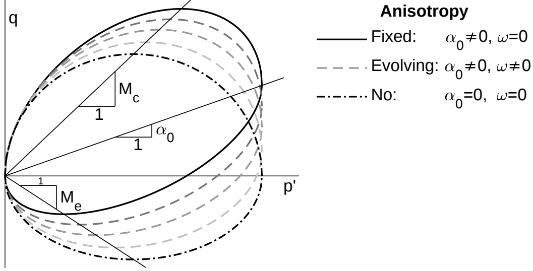
Figure 3.6: Initial surface orientation and evolving surface rotation, with Lode-angle dependency. Adapted from Paper D.
