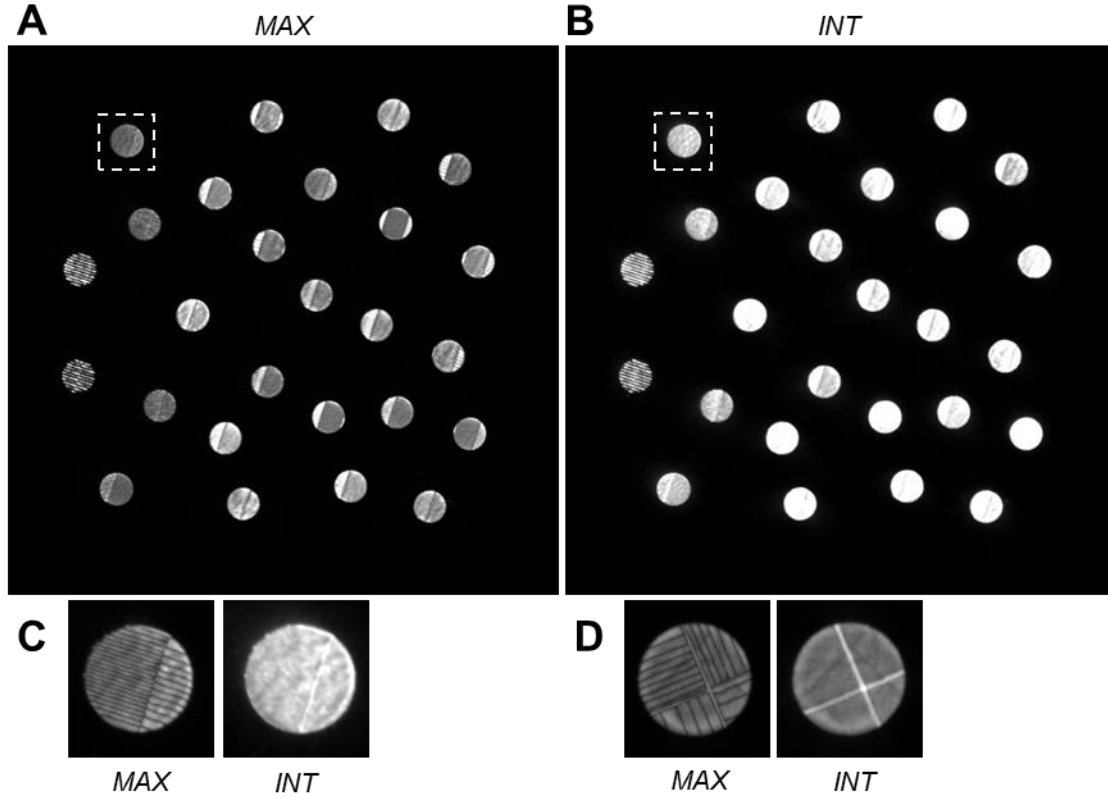
Figure 15: Sample MAX (A) and INT (B) outputs from optical tomography monitoring. The regions highlighted in (A) and (B) are shown in (C); in this case, a stripe hatching pattern was used. A chess hatching pattern was used in the specimens represented in (D).
