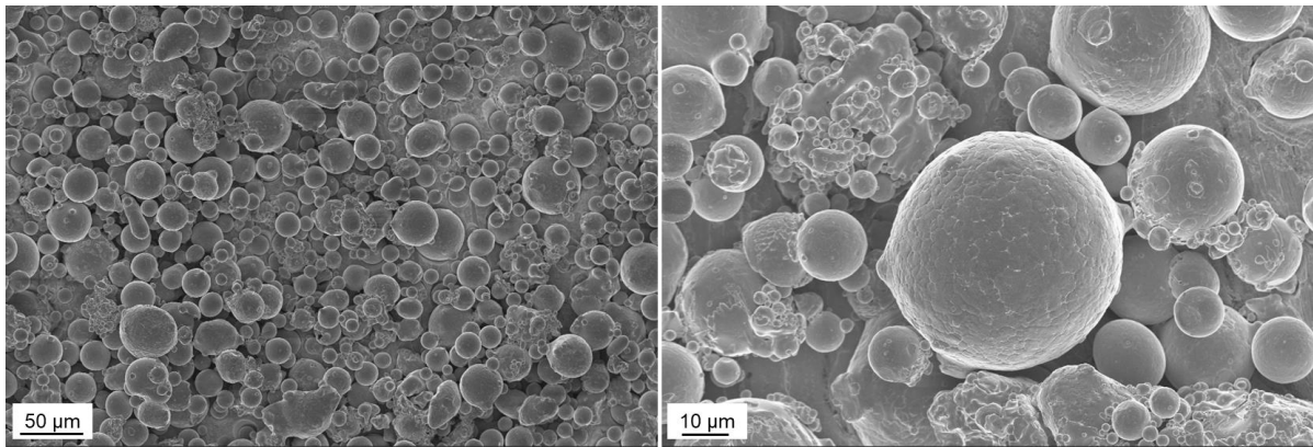
Figure 11: Sample Hastelloy X feedstock powder supplied by EOS GmbH.
