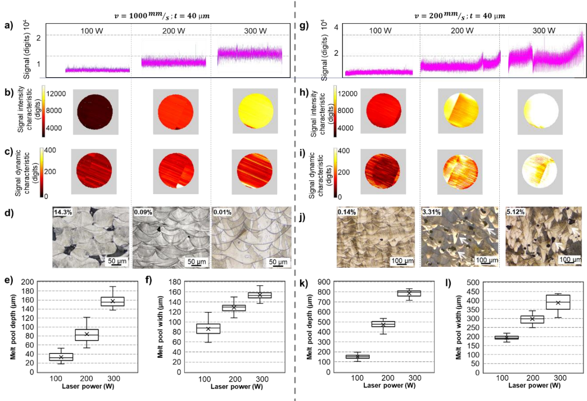
Figure 17: Influence of laser power on melt pool signal characteristics, melt pool dimensions and defect populations in the conduction (a-f) and keyhole regimes (g-l). The specimens were manufactured with varying laser power (100 W, 200 W and 300 W). The plots in a) and g) show the MPM output in temporal x-coordinate. The signal translated to spatial coordinates is shown in b) and h). The signals processed to highlight regions of high melt pool dynamics are shown in c) and i). The microstructures of the corresponding specimens are shown in d) and j), where the volume fraction of defects is indicated. The influence of laser power variation on melt pool depths and widths are shown in e), f), k) and l). Adapted from Paper I 106 .
