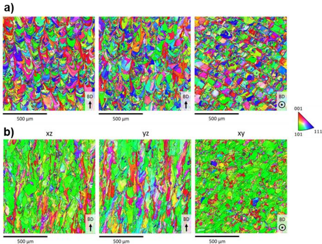
Figure 9: EBSD orientation maps showing the microstructure of Hastelloy X manufactured with different processing conditions in three planes. The build direction (BD) is indicated. Adapted from Paper IV 73 .
