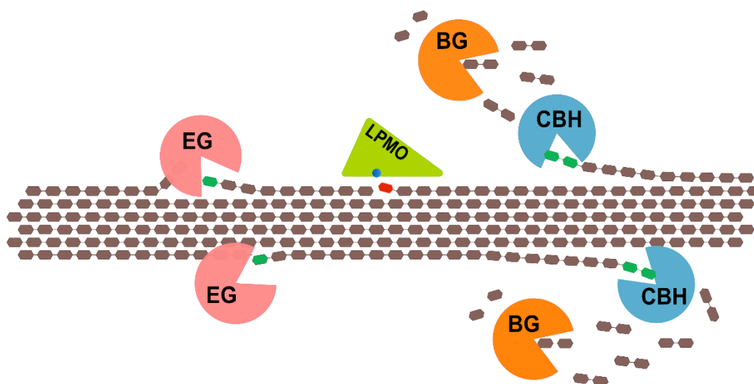
Figure 9. Schematic overview of the model for enzymatic degradation of cellulose. The mode-of-action of LPMOs, endoglucanase, cellobiohydrolase and \beta -1,4-glucosidase are described in the main text. Hydrolysis reactions are represented by coloring the involved glucose monomers/dimers in green. For the oxidative action of LPMOs, red color is used.
