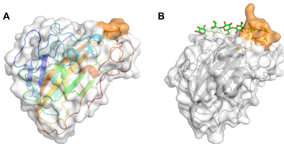
Figure 19. Comparison of the substrate-binding surfaces of McAA9F (A) and CvAA9A (PDB ID: 6yde). The surface area generated by the L3 loop is colored in orange for both enzymes. The ridge on the surface of CvAA9A is evident compared to the flat surface of McAA9F. This ridge has been proposed to be involved in interacting with oligosaccharides, such as cellohexaose, here colored in green.
