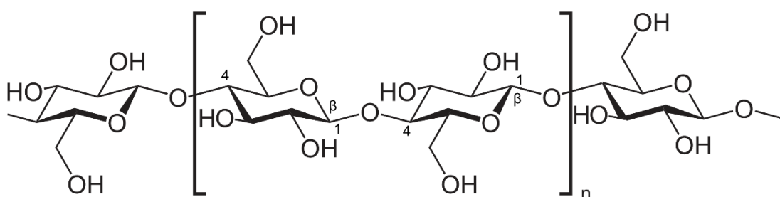
Figure 3. The chemical structure of cellulose, made of monomers of \beta -1,4-D-glucan. In brackets is the smallest repeating unit, cellobiose.
