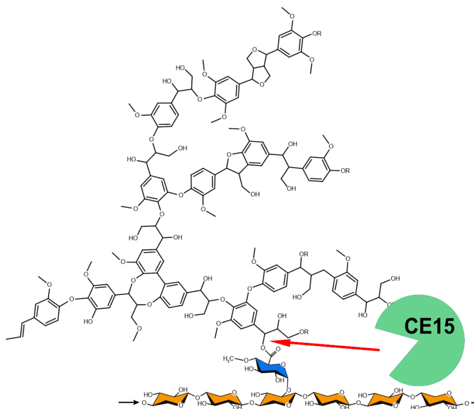
Figure 10. Schematic representation of the action of a CE15 enzyme on the LC bond between glucuronoxylan and lignin. Xylan is colored in orange, GlcA is colored in blue. Figure courtesy of Johan Larbsrink.
