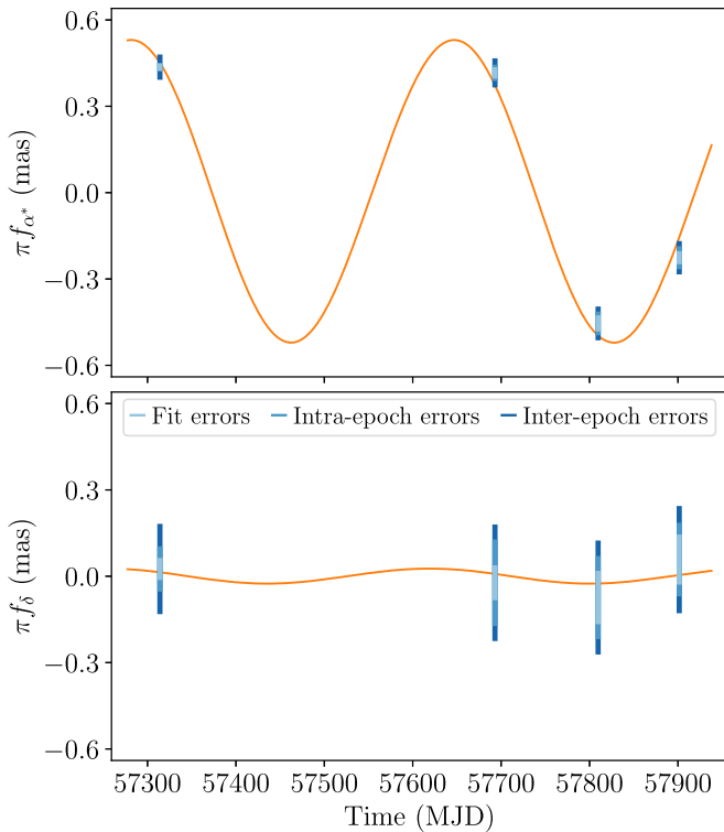
Figure 7. Position residuals in R.A. (top) and decl. (bottom). The best-fit proper motion and relative offset between the Crab Pulsar and SE_CAND3 (see Table 4), after subtracting the best-fit offset at our reference epoch, MJD 57680 (see Table 5). Different colors in the error bars indicate the effects of the additional contributions to the uncertainties (see Table 4).
