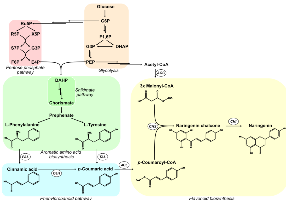
Figure 4. Overview of metabolic pathways involved in flavonoid biosynthesis. The phenylpropanoid acid precursors are derived from AAAs, which are synthesized via the shikimate pathway, using erythro-4-phosphate (E4P) and phosphoenolpyruvate (PEP) as substrates. Malonyl-CoA is derived from acetyl-CoA carboxylation. Flavonoids are generated by a cyclization reaction of a phenylpropanoid acyl-CoA thioester and three malonyl-CoA moieties. ACC: acetyl-CoA carboxylase; PAL: phenylalanine ammonia-lyase; TAL: tyrosine ammonia-lyase; C4H: cinnamate-4-hydroxylase; 4CL: 4-coumarate:CoA ligase; CHS: chalcone synthase; CHI: chalcone isomerase.
