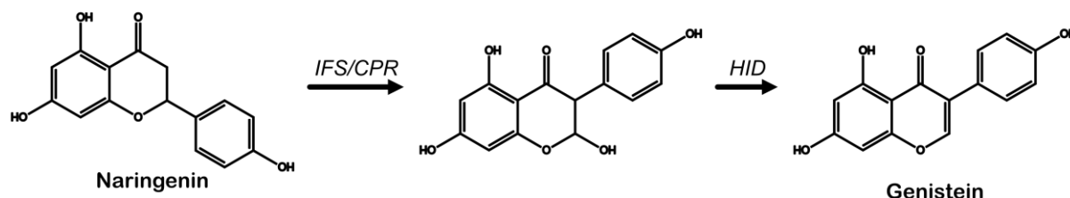
Figure 11. Biosynthetic pathway of naringenin to genistein. The cytochrome P450 enzyme IFS catalyzes the migration of ring B from the C2 to C3 position and requires a cytochrome P450 reductase (CPR) as a redox partner. The dehydration of the resulting intermediate by HID yields genistein.
