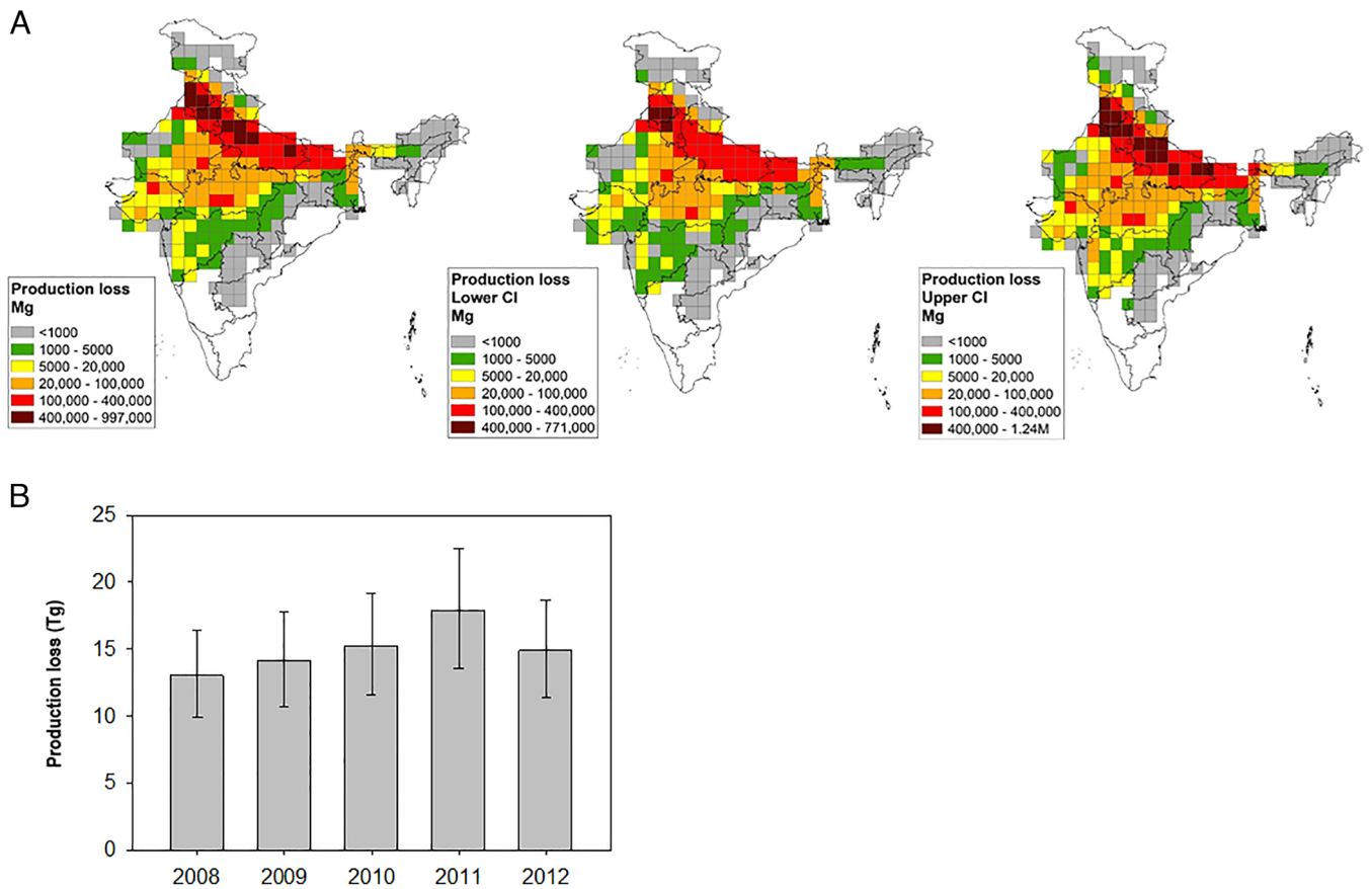
Fig. 1. Wheat production loss due to ozone in India. (A) Mean production loss (in Mg) across India over 2008 to 2012. Lower CI and upper CI represent 95% CI. Wheat production does not occur in white cells. (B) Total production loss in India (in Tg). Error bars represent lower and upper estimates for 95% CI.
