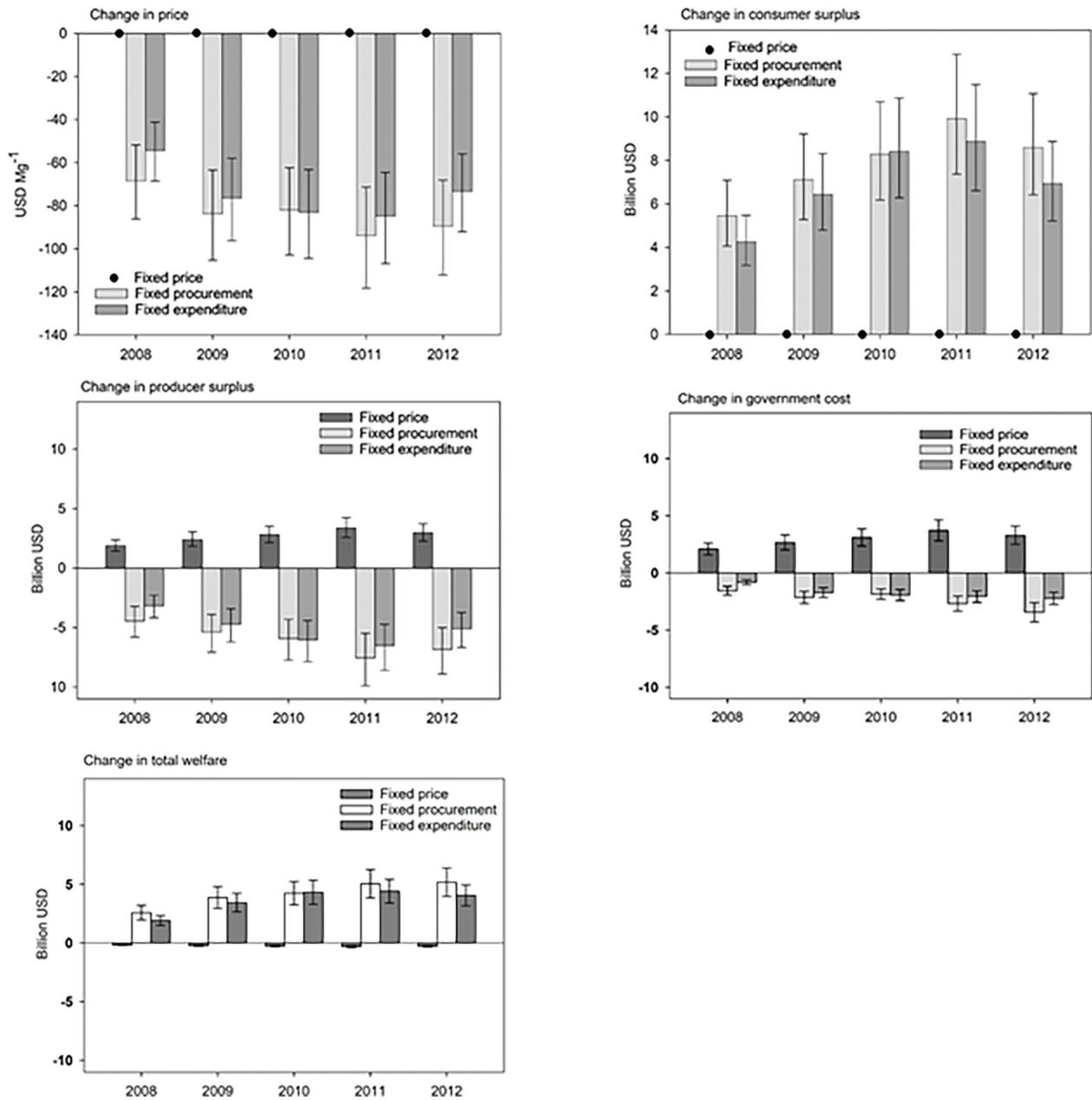
Fig. 4. Changes in the market price of wheat, consumer surplus, producer surplus, government costs, and total welfare in the three policy scenarios resulting from the ozone mitigation with respect to the baseline (ambient ozone pollution). Bars represent the annual mean over 2008 to 2012. Error bars represent lower and upper estimates for the 95% CI. There is no change in market price and consumer surplus in the “fixed-price” scenario due to ozone mitigation.
