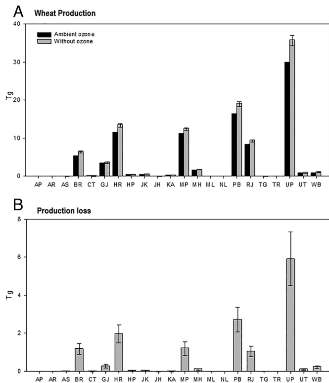
Fig. 2. The wheat production and production loss due to ozone pollution in different states of India under the actual level of irrigation. (A) Production under ambient levels of ozone pollution and without ozone pollution. (B) Total production loss due to ozone pollution. Bars represent mean values over 2008 to 2012; error bars represent 95% CI. AP: Andhra Pradesh, AR: Arunachal Pradesh, AS: Assam, BR: Bihar, CT: Chhattisgarh, GJ: Gujarat, HR: Haryana, HP: Himachal Pradesh, MH: Maharashtra, ML: Meghalaya, NL: Nagaland, PB: Punjab, RJ: Rajasthan, TG: Telangana, TR: Tripura, UP: Uttar Pradesh, UT: Uttarakhand, WB: West Bengal.
