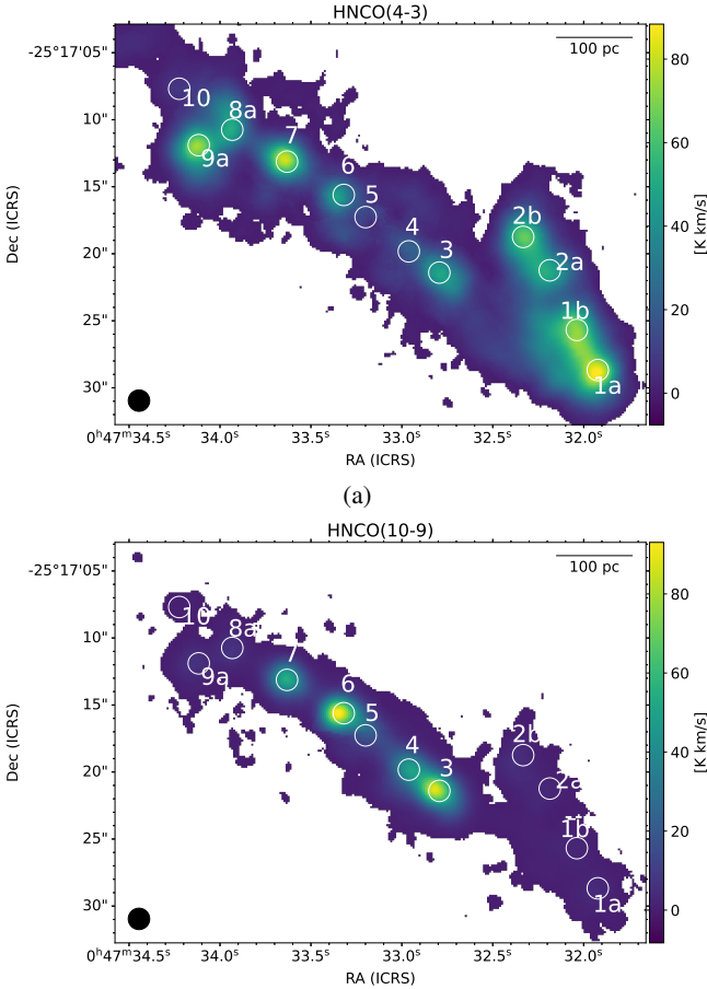
Fig. 1. Velocity-integrated line intensities in [\text{K km s}^{-1}] of the HNC0 transitions: ( 4^{0.4-3^{0.5}} ) and ( 10^{0.10-9^{0.9}} ), in (a) and (b), respectively. These two transitions are representative of the drastic variation in the trend of brightness from outer to inner GMCs. The rest of the HNC0 line intensity maps are provided in Appendix B. The studied GMC regions as listed in Table 2 are labeled in white text on the map. The ALCHEMI 1''.6 \times 1''.6 beam is displayed in the lower-left corner of the map.
