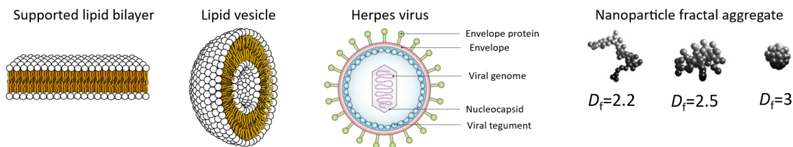
Figure 2 Selection of the biological structures and particles investigated in the papers appended to this thesis, which includes supported lipid bilayers (SLBs), lipid vesicles, herpes viruses, and nanoparticle aggregates. D_f is the fractal dimension, where a lower D_f corresponds to fewer particles per unit volume in an aggregate. The images of the fractal aggregates are adapted from Ref. [56] under CC-BY license.
