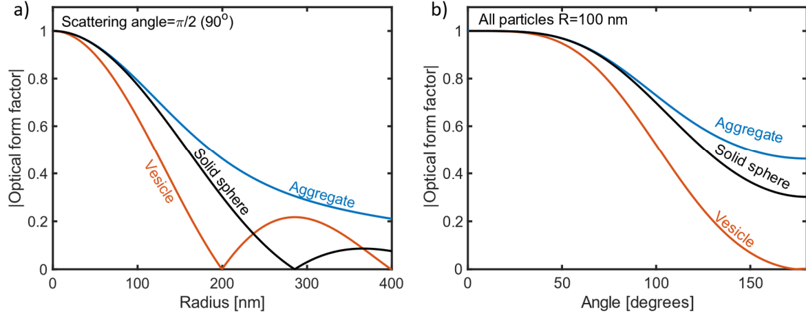
Figure 5 The optical form factor from Rayleigh-Debye-Gans theory for homogenous spheres, lipid vesicles, and aggregates with a fractal dimension of 2 using a wavelength of 532 nm and a surrounding medium refractive index of 1.33. The optical form factor as a function of (a) size when the scattering angle is 90 degrees and (b) as a function of scattering angle for a particle with a radius of 100 nm.
