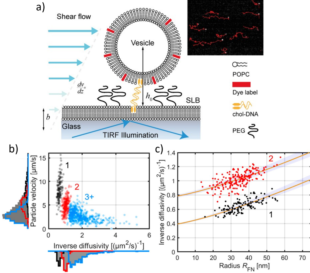
Figure 18 Two-dimensional flow nanometry (2DFN) of tethered vesicles and the subsequent data analysis. (a) Illustration of the 2DFN concept. Labelled vesicles are linked to a supported lipid bilayer (SLB) using cholesterol-DNA-tethering within a microfluidic channel. A shear-flow is applied and the two-dimensional movement of the vesicles are tracked using fluorescence microscopy. b indicates the potential slip length of the SLB and h_0 is the distance from the centre of the particle to the SLB. Inset: fluorescence micrograph showing the shearing of vesicles in the field of view with tracks highlighted in red. (b) Flow induced particle velocity versus inverse diffusivity for POPC liposomes tethered to and SLB consisting of POPC. The different colours indicate the number of tethers (1, 2 and 3+). (c) Inverse diffusivity versus R_{FN} for the first two vesicle-tether clusters in (b). The estimated values from the least-square fit (yellow lines) are b_{ef} = 22.8 \pm 6.3 nm and D_T = 2.56 \pm 0.07 \mu\text{m}^2/\text{s} (mean \pm 95% CI, visualised using the shaded blue region). Adapted from [206] under CC-BY license.
