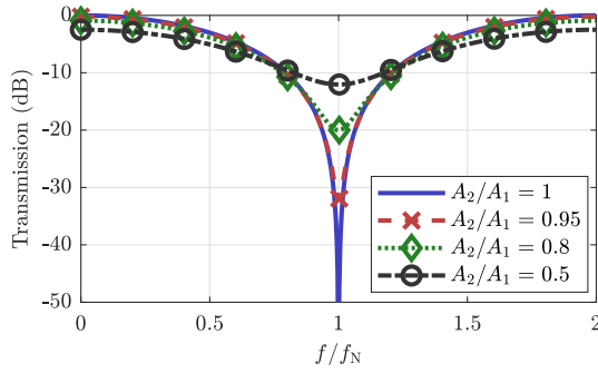
FIGURE 9 Transmission magnitude |A_{out}|/|S_{in}| as a function of f/f_N when A_1 = 1/\sqrt{2} for different amplitude ratios A_2/A_1 .
