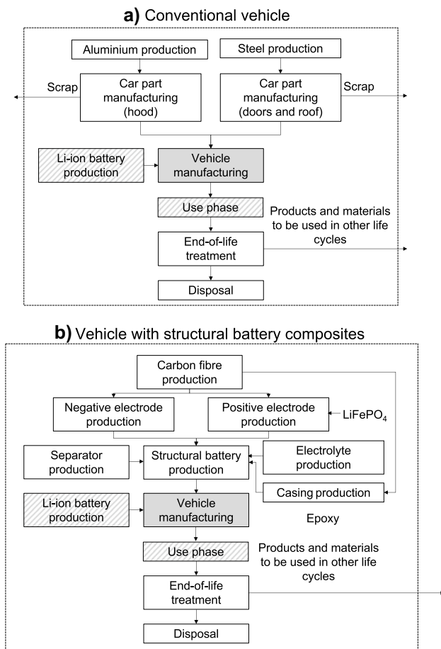
Fig. 3 The basic outline for the cradle-to-grave life cycle of the vehicle. The figure shows the main processes for the considered vehicle parts for a conventional battery electric vehicle (a) and a battery electric vehicle with structural battery composites (b). The lithium-ion battery production and the use phase (striped boxes) are only partly included as this is a comparative assessment. The vehicle manufacturing (grey box) is not included in the assessment (assumed to be similar for both vehicles)
