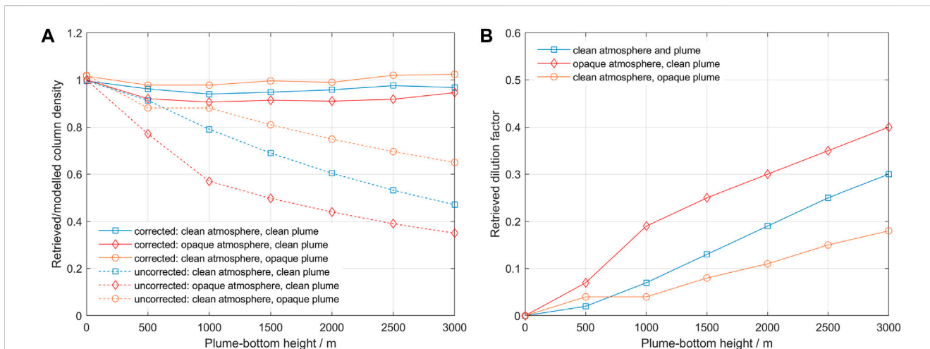
FIGURE 8 (A) Retrieved/modelled column density as a function of altitude for the three modelled cases. The results without correction are shown with dashed lines, and the results after the correction are shown with continuous lines. (B) Retrieved dilution factor as a function of altitude for the three modelled cases.
