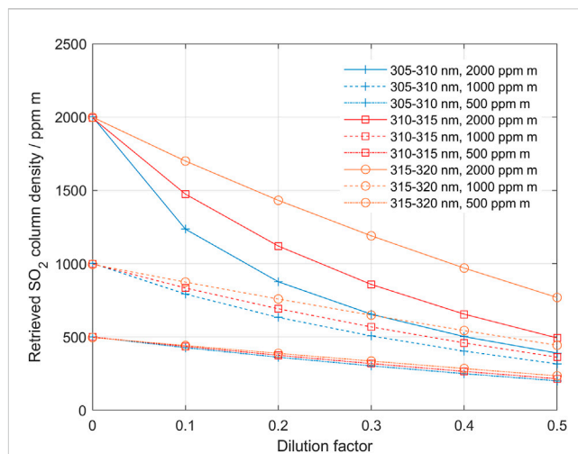
FIGURE 4 The underestimation of derived SO_2 column as a function of dilution, when using the different evaluation bands; 305–310 nm (blue), 310–315 nm (red) and 315–320 nm (orange) for SO_2 columns of 500, 1,000 and 2,000 ppm m, respectively. By following a pair of evaluated columns from high to low dilution the behavior of the iterative process in the dilution correction algorithm can be studied (see, for example Figure 3 above and Figure 11 below).
