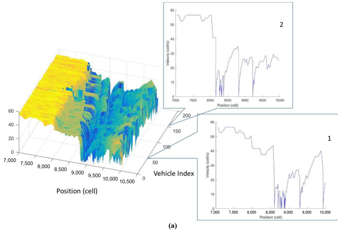
Figure 11 Velocities over locations around the work zone
