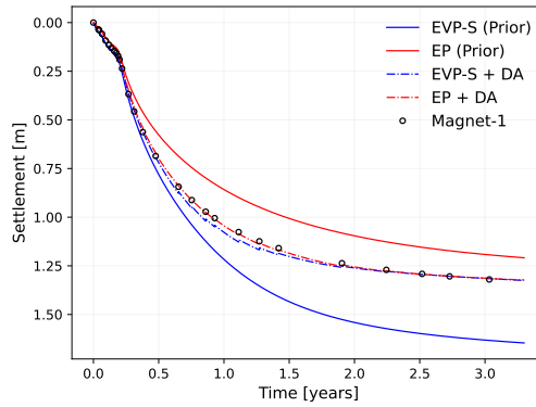
Figure 5.8: Comparison of the data assimilated state predictions with that from prior knowledge for the EP and EVP-S models.
