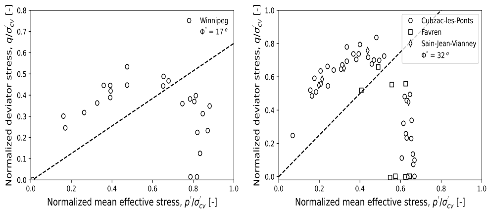
Figure 2.1: Yield points of different natural soft soils (reproduced from (Lämsivaara, 1999)).
