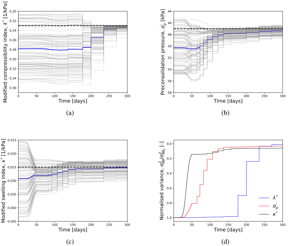
Figure 5.6: Convergence of particles of EnKF (0–300 d) for Elastoplastic model parameters in (a),(b),(c) [Color representation: Solid Gray: ensemble, Solid Blue: mean of the ensemble, Dashed black: Synthetic true value] and (d) normalised variance of all parameters.
