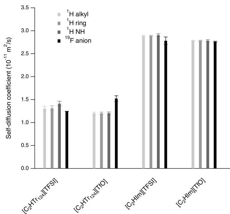
Figure 4. Self-diffusion coefficients estimated from PFG NMR measurements for different 1 H and 19 F resonances and for all four protic ionic liquids at 34 °C. The errors show the standard deviation of the fitted diffusion coefficient.
