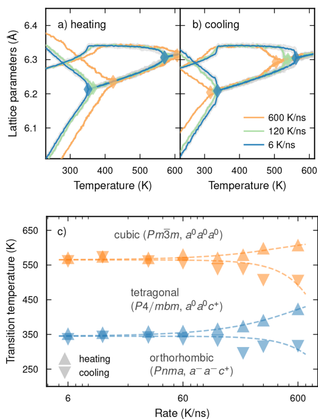
Figure 1. Convergence with heating/cooling rate. Lattice parameters for CsPbI 3 as a function of temperature from MD simulations with varying (a) heating and (b) cooling rates for supercells comprising 61440 atoms. The transition temperatures extracted from these data are indicated by diamonds. The gray lines show the raw data, whereas the colored lines show the data after application of a Hamming window of 0.6 K (see Figure S4). (c) Transition temperatures as a function of heating/cooling rate. Dashed lines are guides to the eye. All results were obtained using the full model (see the “Model Construction” section) based on the vdW-DF-cx exchange-correlation functional.
