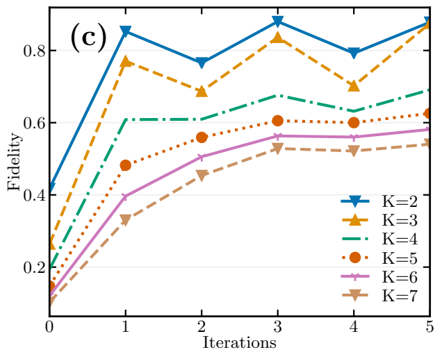
FIG. 14. Fidelity to a target qunaught state with squeezing \Delta = 0.4 as a function of the number of iterations for binomial input states with rotational symmetry of order (a) N = 2 , (b) N = 3 , and (c) N = 4 , and for K = 2-7 for each N .
