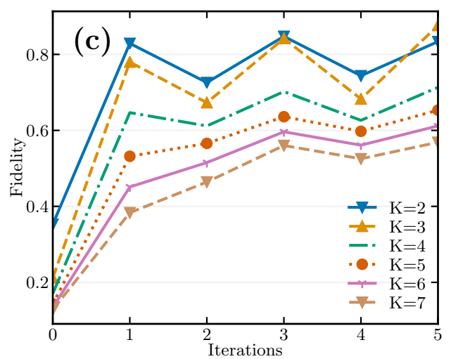
FIG. 15. Fidelity to a target qunaught state with squeezing \Delta = 0.35 as a function of the number of iterations for binomial input states with rotational symmetry of order (a) N = 2 , (b) N = 3 , and (c) N = 4 , and for K = 2-7 for each N .
