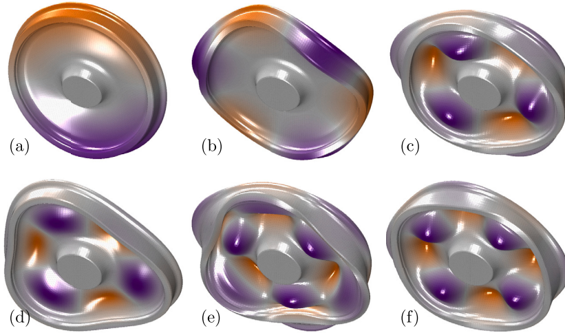
Fig. 4. Vibrational mode shapes: (a): (1, 0, a) at 160 Hz, (b): (3, 0, a) at 834 Hz, (c): (3, 1, a) at 2120 Hz, (d): (3, 0, r) at 2503 Hz, (e): (3, 2, a) at 3467 Hz, (f): (4, 1, a) at 2545 Hz. The colour indicates axial deflection. (For interpretation of the references to colour in this figure legend, the reader is referred to the web version of this article.)
