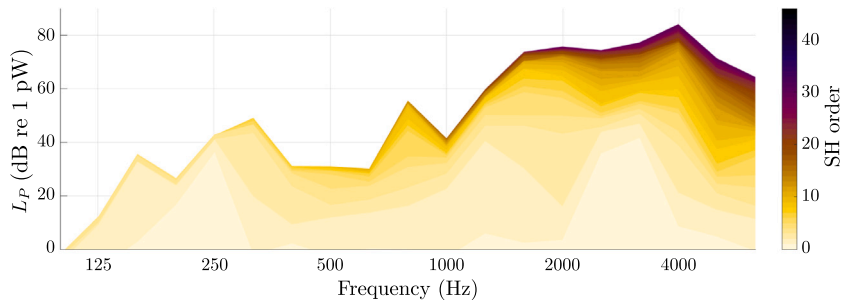
Fig. 8. Predicted sound power in third-octave bands on the 5 m sphere as a function of the SH order.
