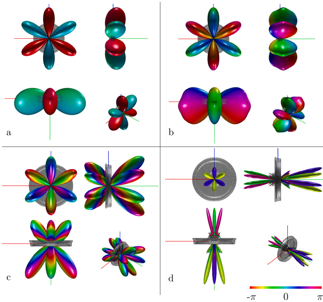
Fig. 11. Directivity of the radial mode (3, 0, r) for (a) 63 Hz, (b) 250 Hz, (c) 1000 Hz, and (d) 4000 Hz. The eigenfrequency of the mode is at 2503 Hz. (For interpretation of the references to colour in this figure legend, the reader is referred to the web version of this article.)
