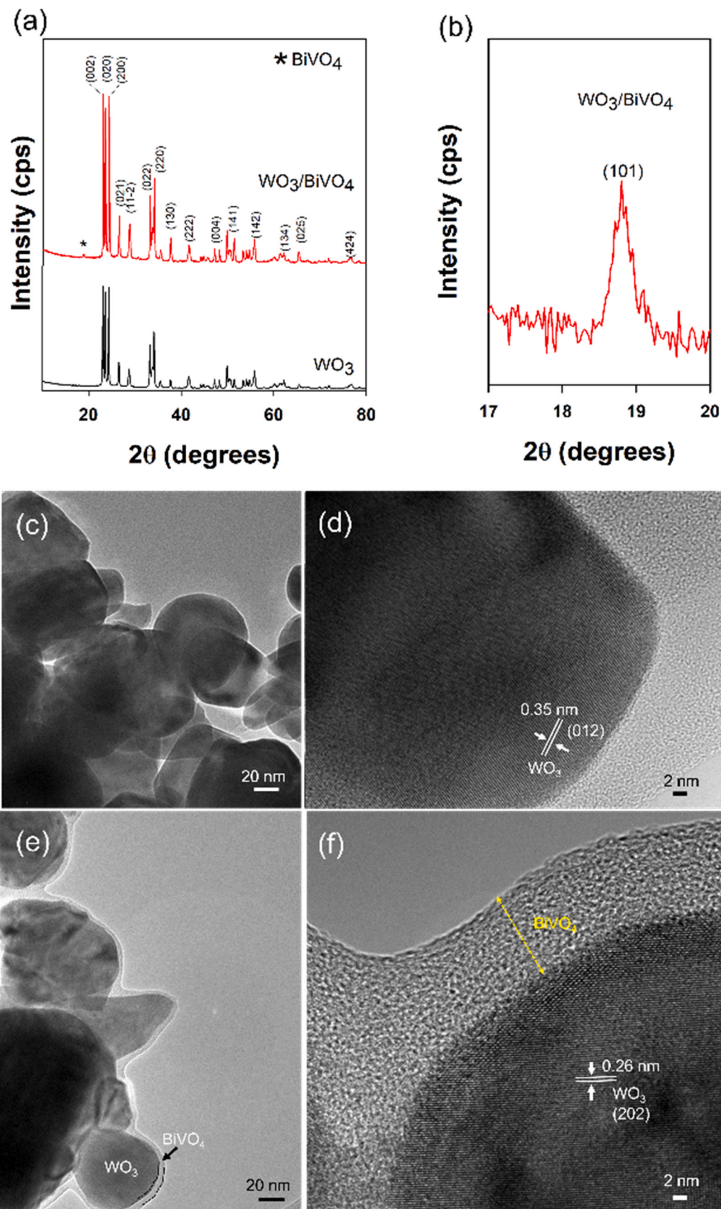
Fig. 1. (a) X-ray diffraction patterns of WO 3 and WO 3 /BiVO 4 films coated onto FTO substrate, (b) Magnified view of X-ray diffraction patterns observed from Fig. 1 (a) for clear eye guidance. HR-TEM images of WO 3 film at (c) 20 nm and (d) 2 nm. HR-TEM images of WO 3 /BiVO 4 films at (e) 20 nm and (f) 2 nm.
