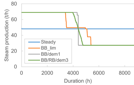
(b) Bark boiler steam production.
