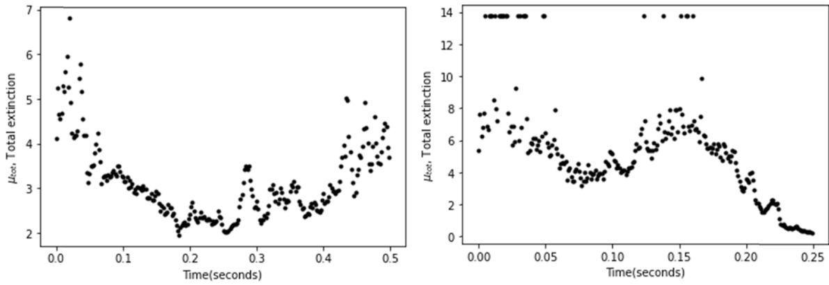
Figure 7. Measured total extinction for the heptane (a) and diesel flame (b), respectively.
