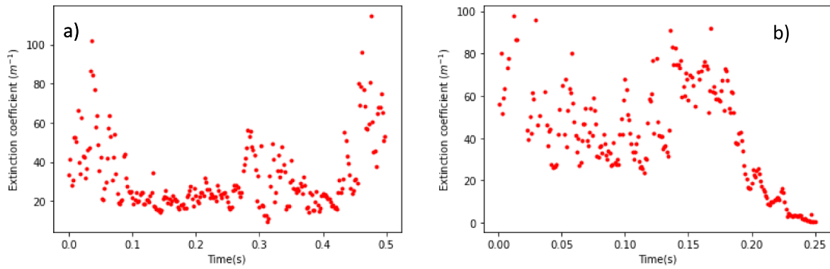
Figure 8. Measured extinction coefficients for the heptane (a) and diesel flame (b).
