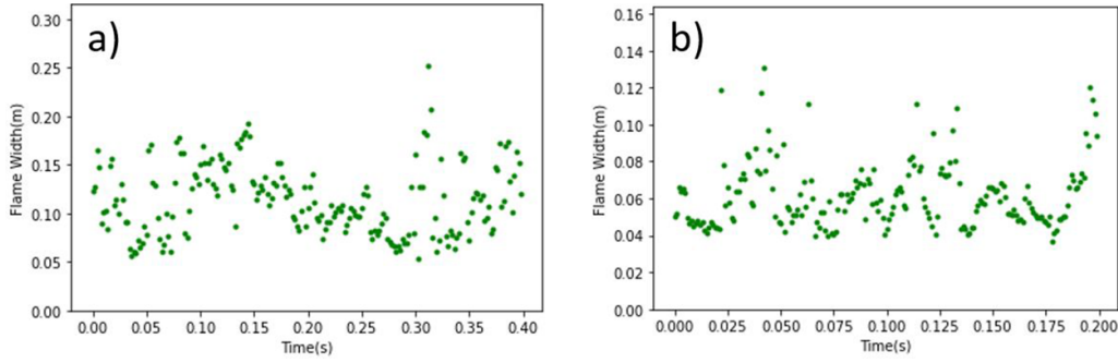
Figure 6. Measured flame size along the laser beam for the heptane (a) and diesel flame (b).
